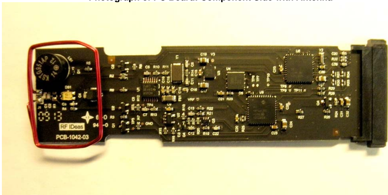
Photograph of PC Board: Component Side with Antenna
