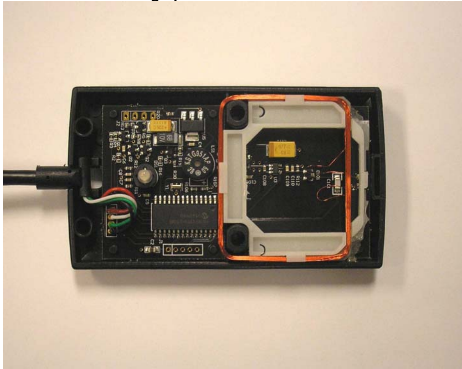
Photograph of EUT Cover Removed
