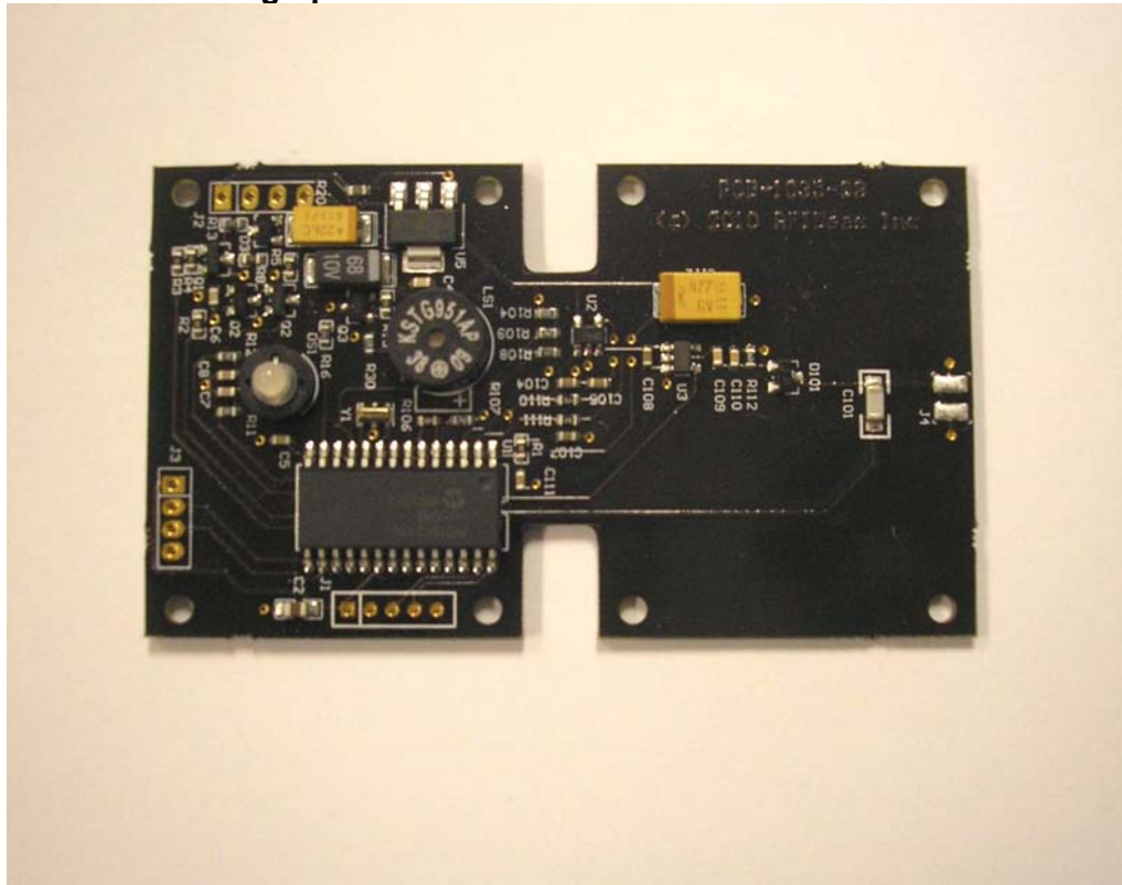
Photograph of Processor board – Antenna removed
