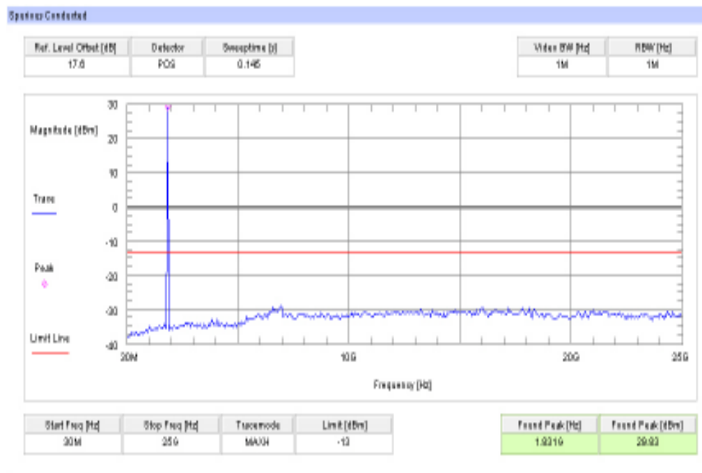
Plot 1: Channel 512 (30 MHz - 25 GHz)
