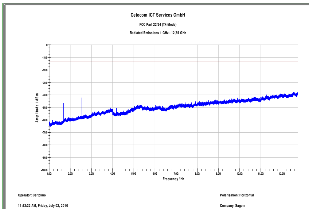
Plot 9: TX mode, channel 189, 1 GHz to 12.75 GHz, horizontal polarization
