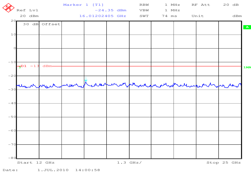
Plot 10: TX mode, channel 661, 12 GHz to 25 GHz, vertical &amp; horizontal polarization
