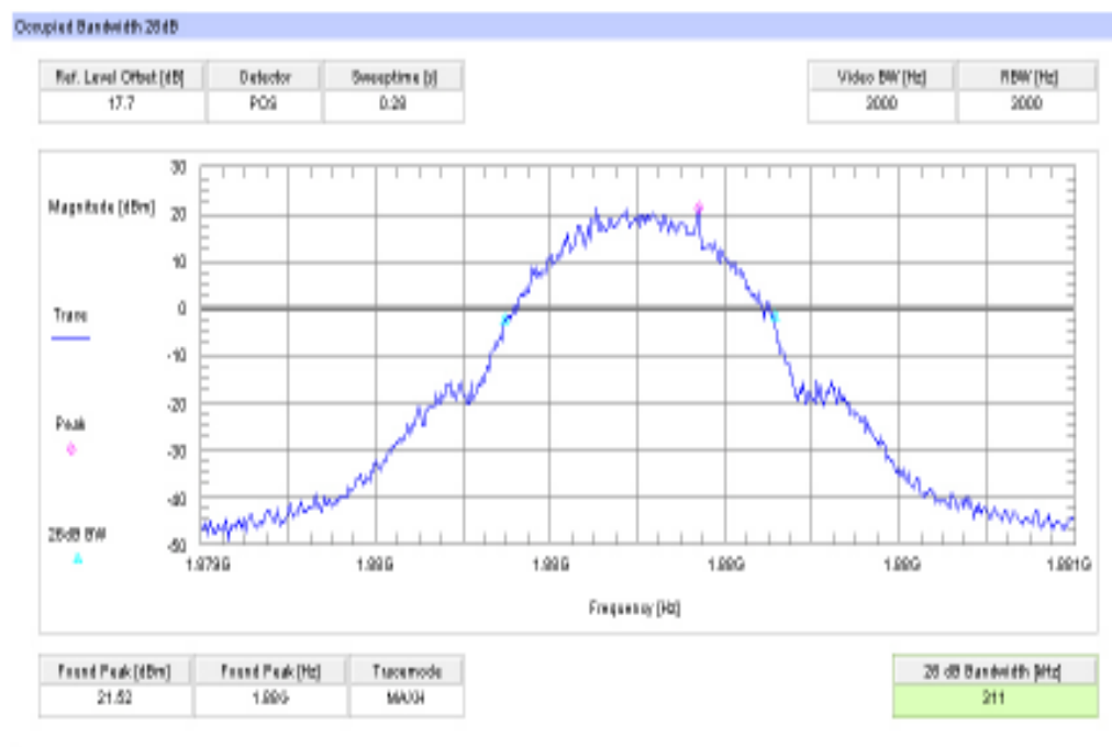
Plot 4: Channel 661 (-26 dBc BW) GSM
