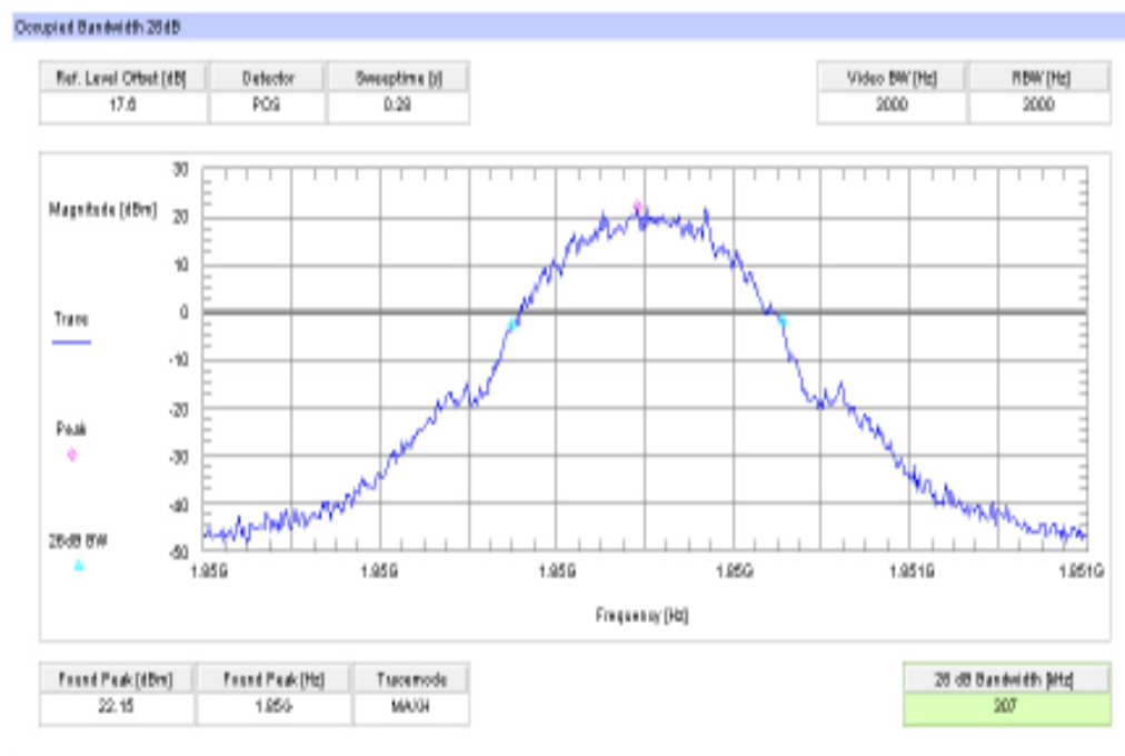
Plot 2: Channel 512 (-26 dBc BW) GSM
