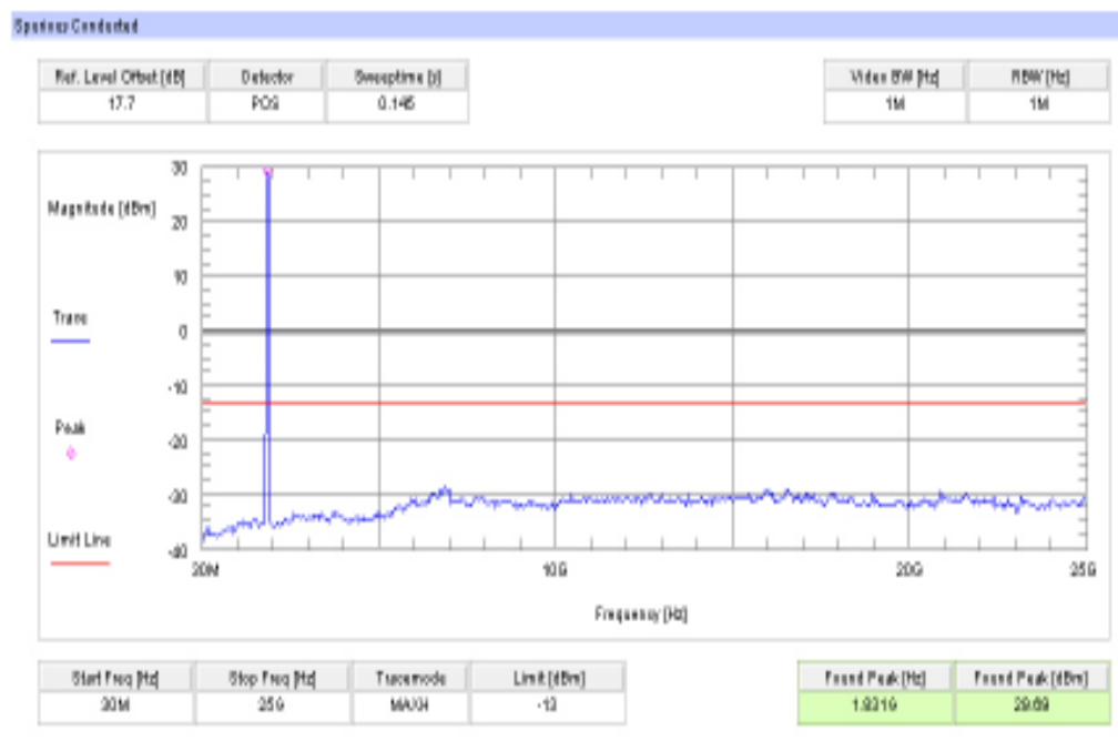
Plot 2: Channel 661 (30 MHz - 25 GHz)
