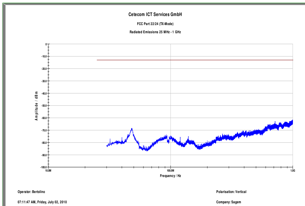
Plot 6: TX mode, channel 661, 30 MHz to 1 GHz, vertical polarization
