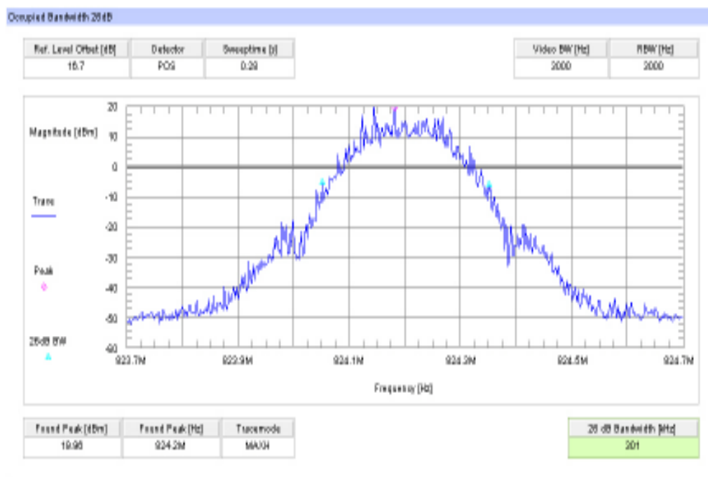
Plot 8: Channel 128 (-26 dBc BW) EGPRS / EDGE
