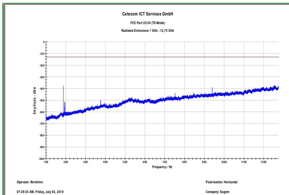
Plot 9: TX mode, channel 661, 1 GHz to 12.75 GHz, horizontal polarization
