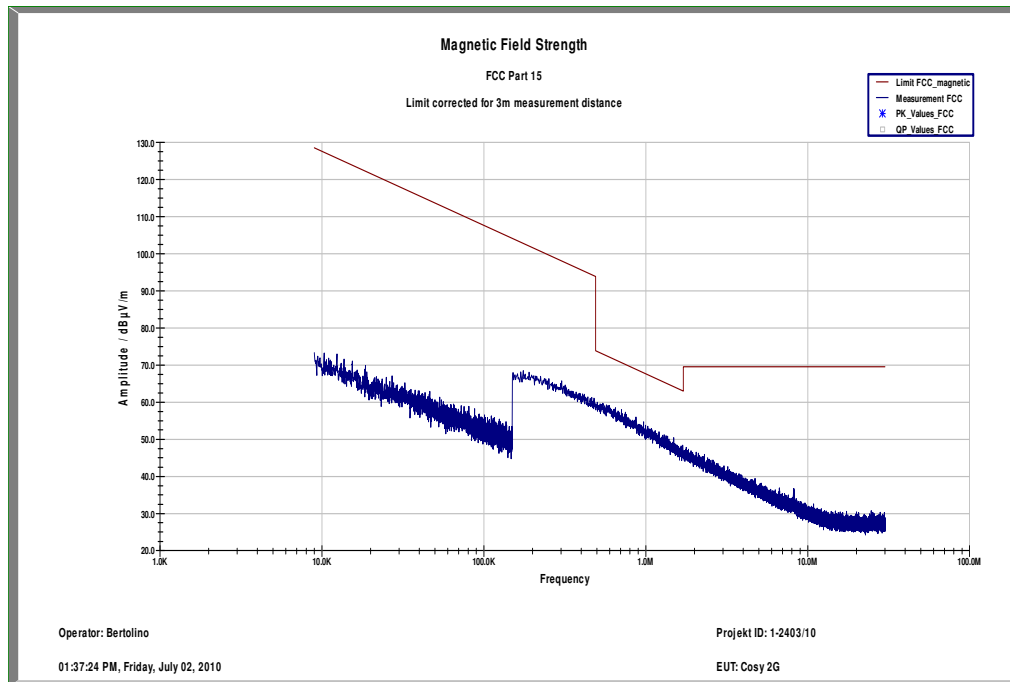
Plot 5: TX mode, channel 661, up to 30 MHz
