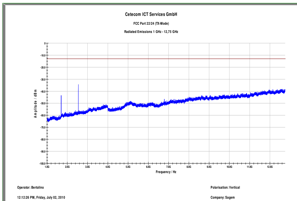
Plot 12: TX mode, channel 251, 1 GHz to 12.75 GHz, vertical polarization
