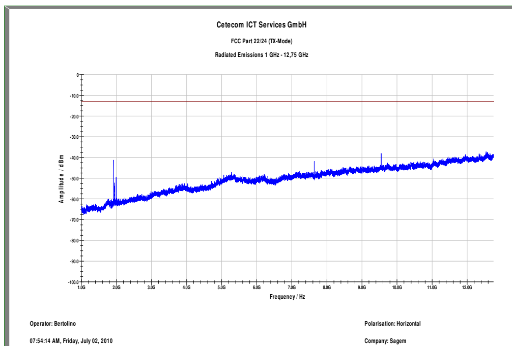
Plot 14: TX mode, channel 810, 1 GHz to 12.75 GHz, horizontal polarization
