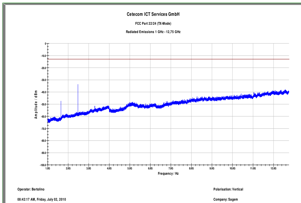
Plot 2: TX mode, channel 128, 1 GHz to 12.75 GHz, vertical polarization
