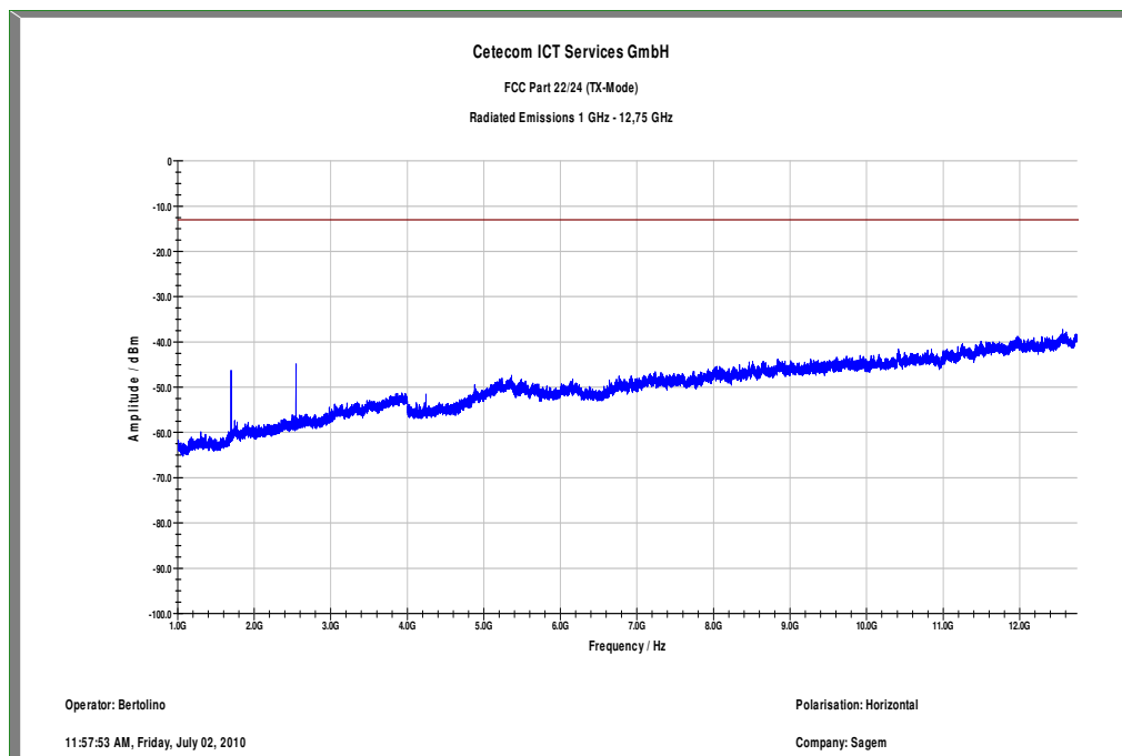
Plot 14: TX mode, channel 251, 1 GHz to 12.75 GHz, horizontal polarization
