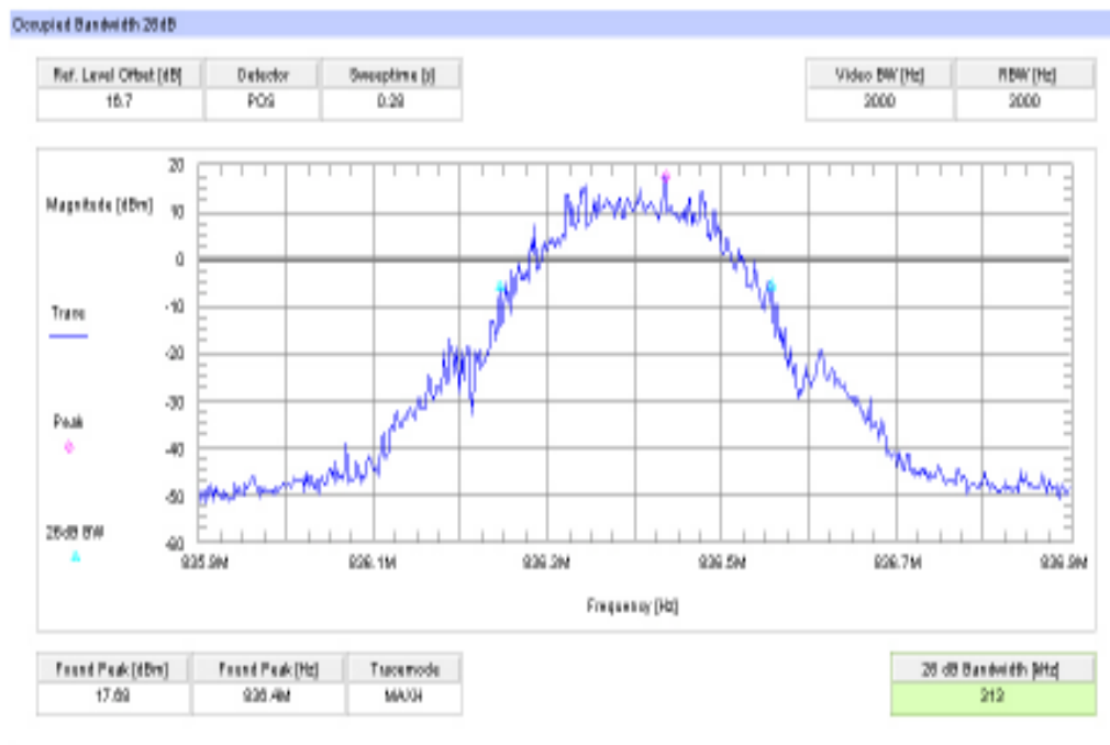
Plot 10: Channel 189 (-26 dBc BW) EGPRS / EDGE
