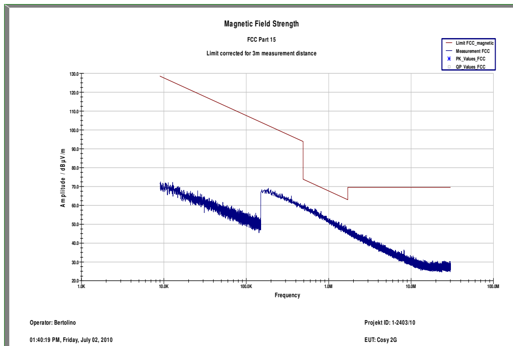
Plot 5: TX mode, channel 189, up to 30 MHz
