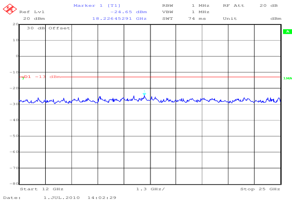
Plot 10: TX mode, channel 189, 12 GHz to 25 GHz, vertical & horizontal polarization
