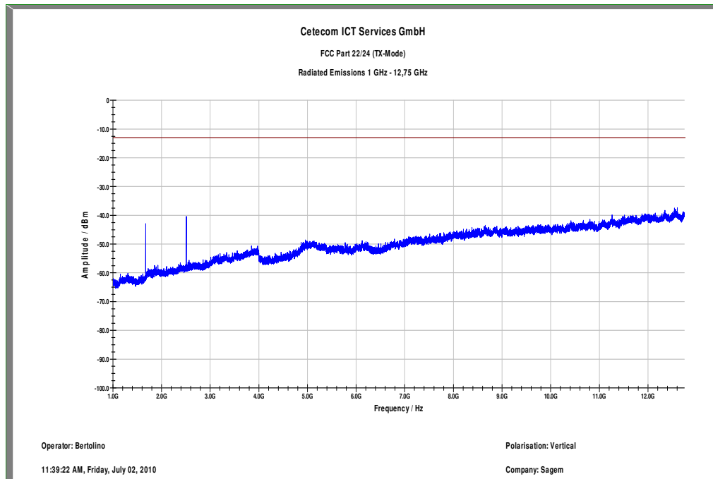
Plot 7: TX mode, channel 189, 1 GHz to 12.75 GHz, vertical polarization
