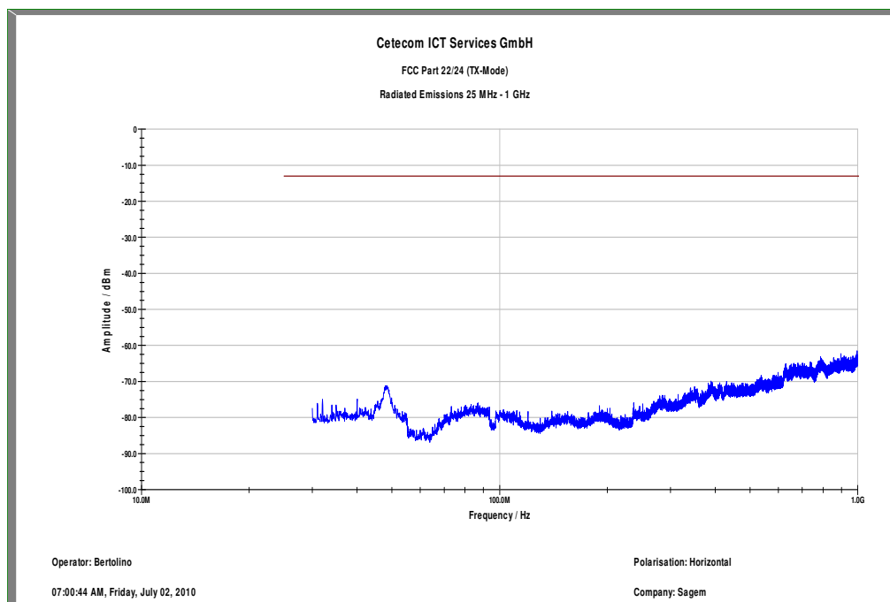
Plot 3: TX mode, channel 512, 30 MHz to 1 GHz, horizontal polarization
