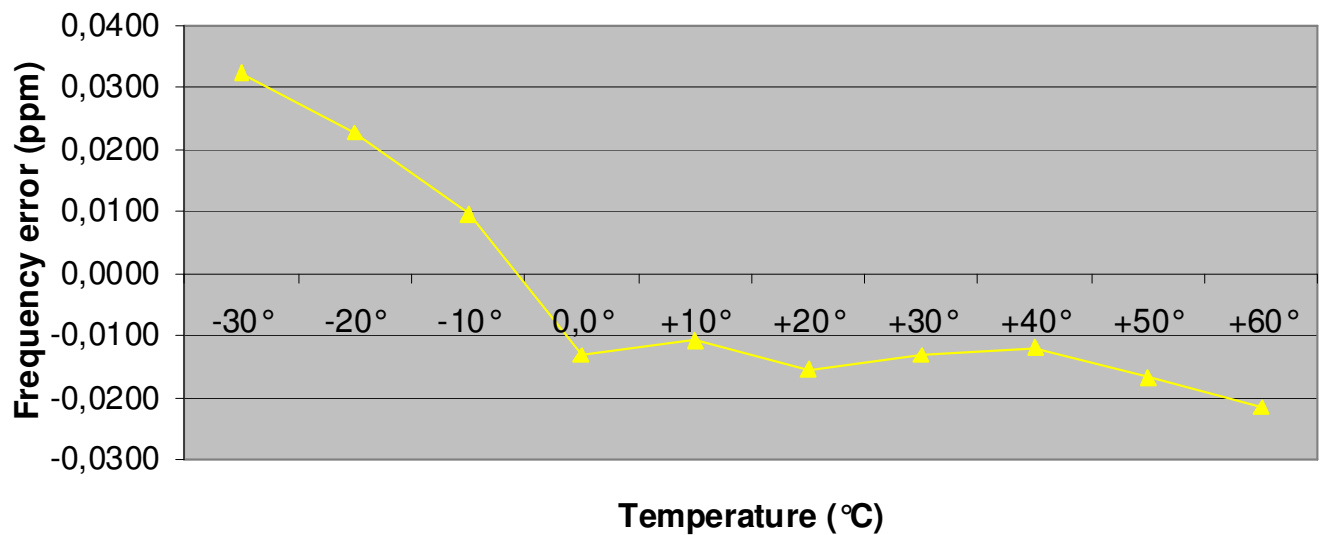
Frequency Error vs. Temperature
