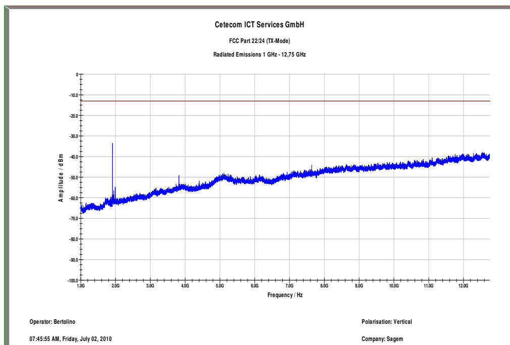
Plot 12: TX mode, channel 810, 1 GHz to 12.75 GHz, vertical polarization
