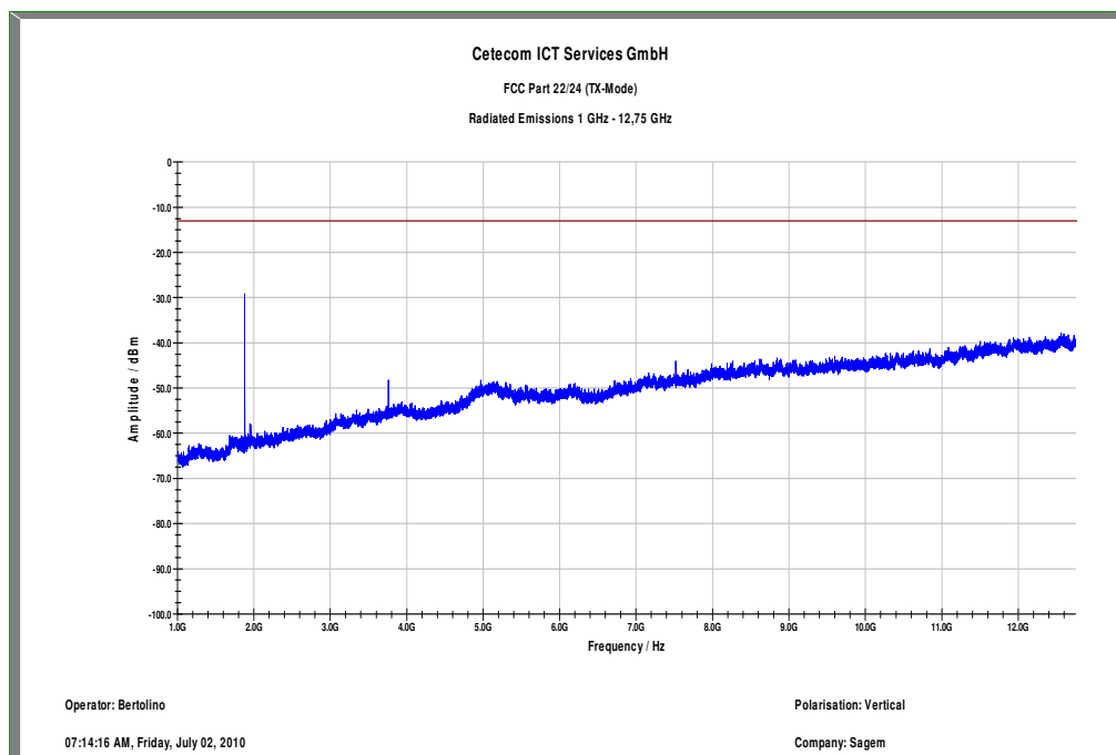
Plot 7: TX mode, channel 661, 1 GHz to 12.75 GHz, vertical polarization
