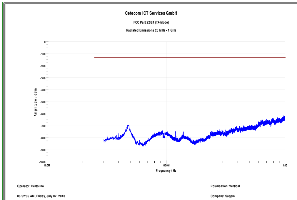
Plot 1: TX mode, channel 512, 30 MHz to 1 GHz, vertical polarization
