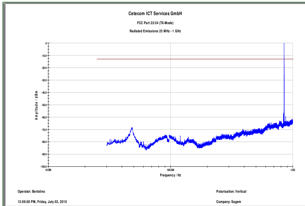
Plot 11: TX mode, channel 251, 30 MHz to 1 GHz, vertical polarization
