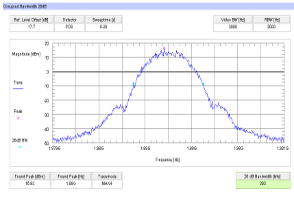
Plot 10: Channel 661 (-26 dBc BW) EGPRS / EDGE
