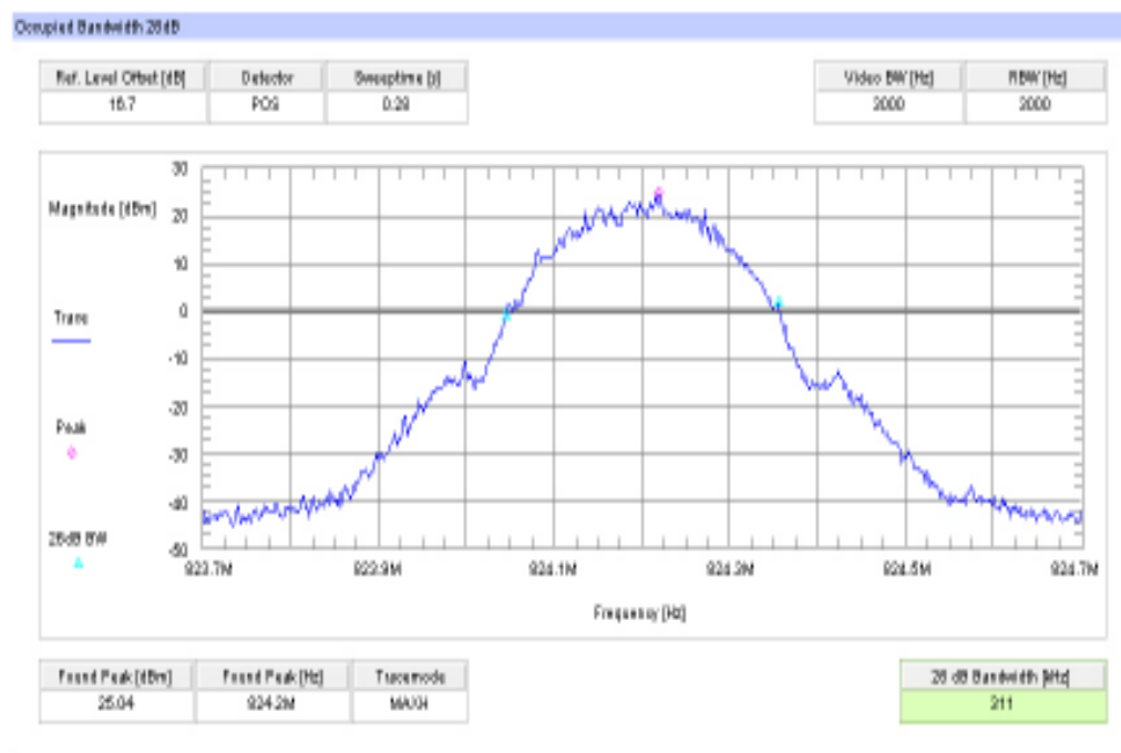
Plot 2: Channel 128 (-26 dBc BW) GSM
