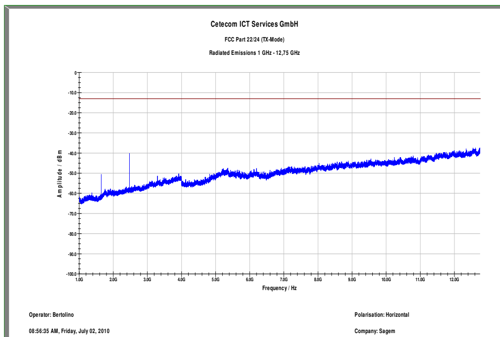
Plot 4: TX mode, channel 128, 1 GHz to 12.75 GHz, horizontal polarization
