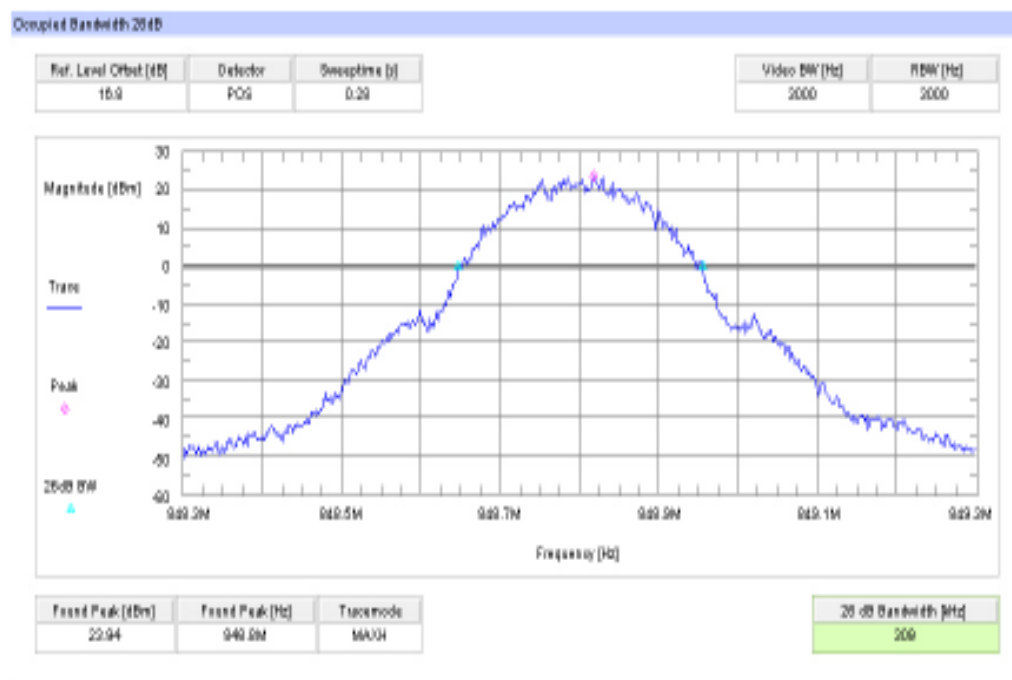
Plot 6: Channel 251 (-26 dBc BW) GSM
