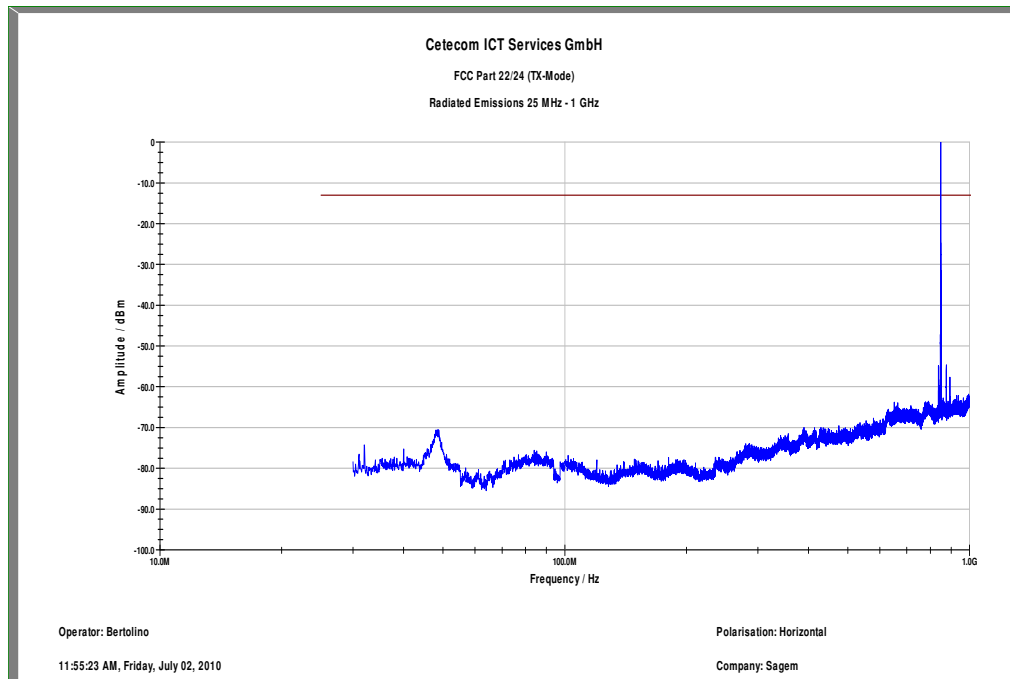
Plot 13: TX mode, channel 251, 30 MHz to 1 GHz, horizontal polarization
