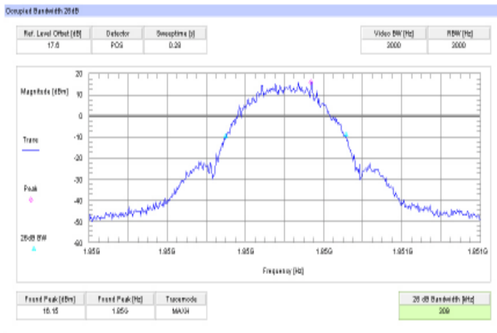
Plot 8: Channel 512 (-26 dBc BW) EGPRS / EDGE
