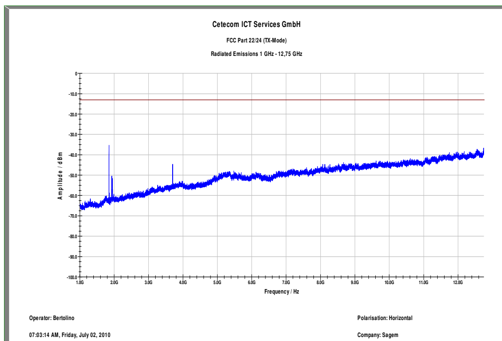
Plot 4: TX mode, channel 512, 1 GHz to 12.75 GHz, horizontal polarization
