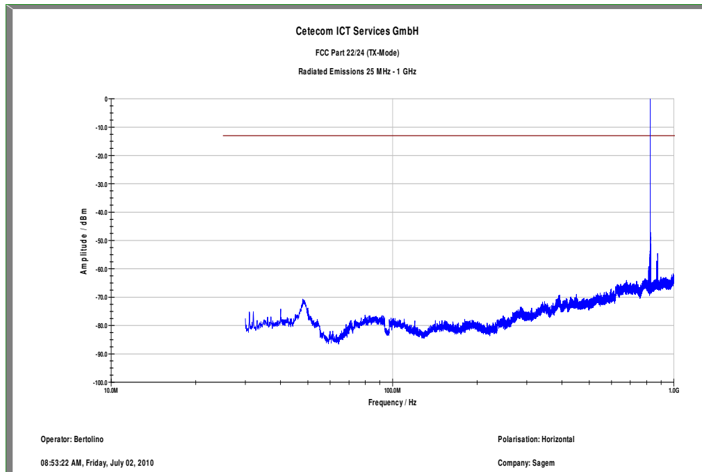
Plot 3: TX mode, channel 128, 30 MHz to 1 GHz, horizontal polarization
