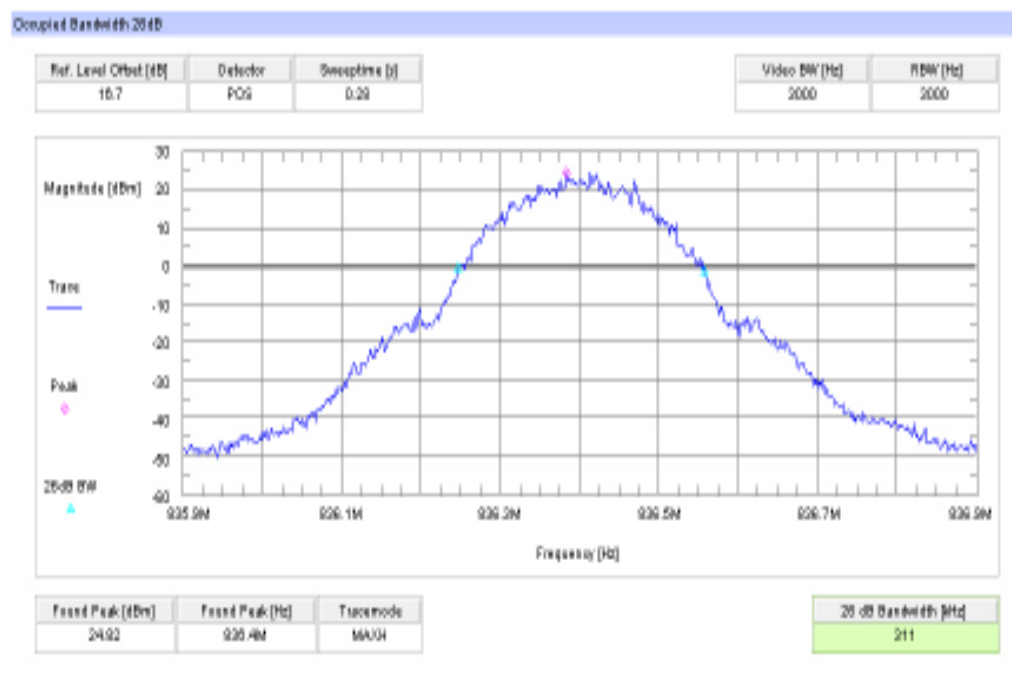
Plot 4: Channel 189 (-26 dBc BW) GSM
