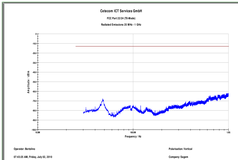
Plot 11: TX mode, channel 810, 30 MHz to 1 GHz, vertical polarization
