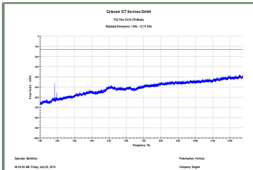
Plot 2: TX mode, channel 512, 1 GHz to 12.75 GHz, vertical polarization
