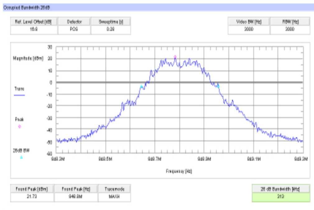
Plot 12: Channel 251 (-26 dBc BW) EGPRS / EDGE
