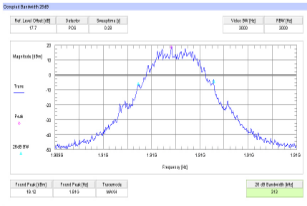
Plot 12: Channel 810 (-26 dBc BW) EGPRS / EDGE
