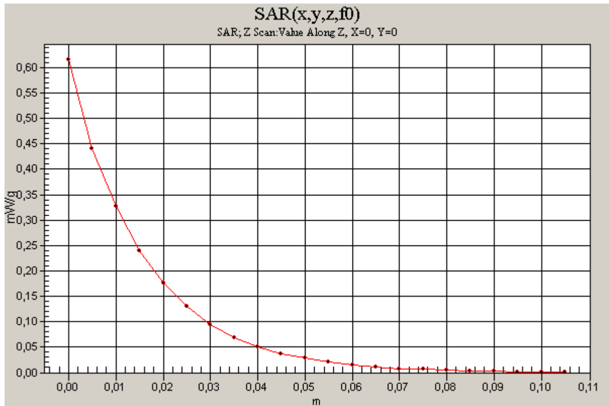
850 MHz head
