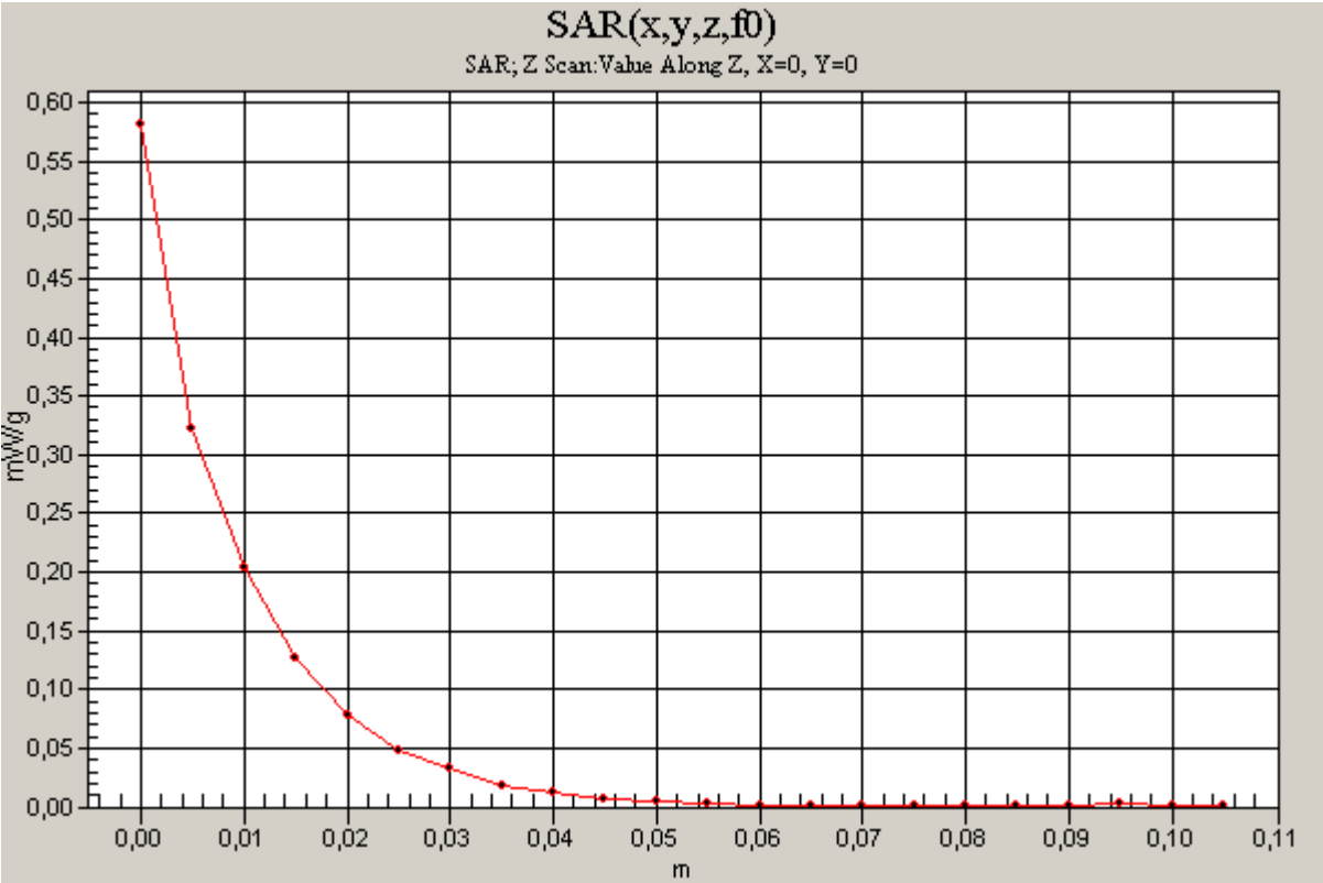
1900 MHz head
