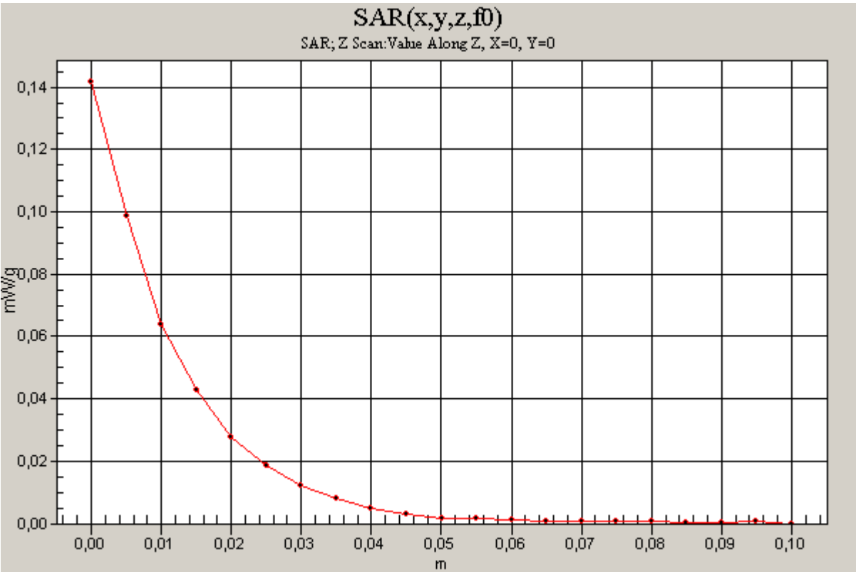
1900 MHz body
