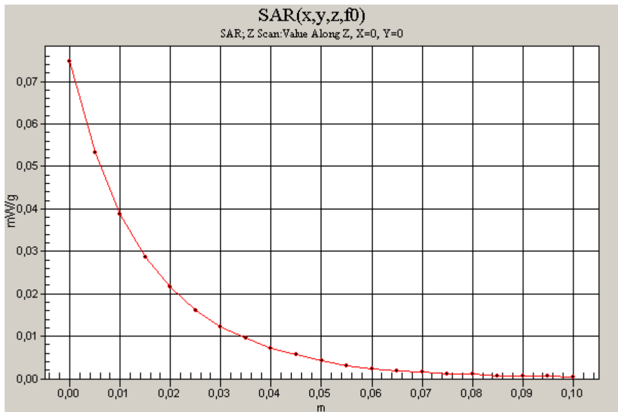
850 MHz body
