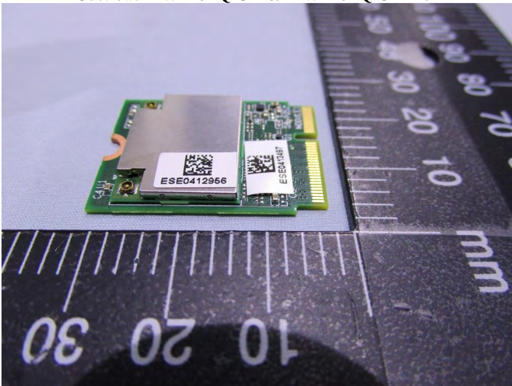
Outview: AIW-173BQ-GI1 & AIW-173BQ-GI2 Pic 4
