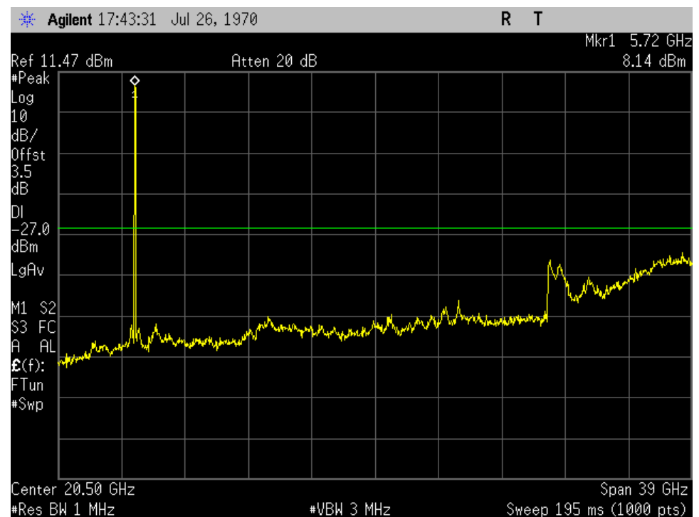
U-NII-3_5745MHz_Low Ch_149_20MHz BW_a-mode_-27dBm_1-40GHz_Port 2
