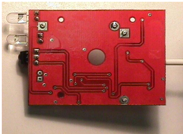
Bottom View of the Point Six IR Door Transmitter Circuit Board, Model Point Sensor IR Door
