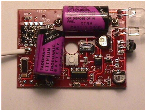
Top View of the Point Six IR Door Transmitter Circuit Board, Model Point Sensor IR Door
