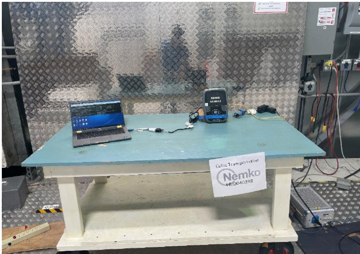
Figure 8.2.1 Conducted disturbance at AC mains port setup photo (Front)
