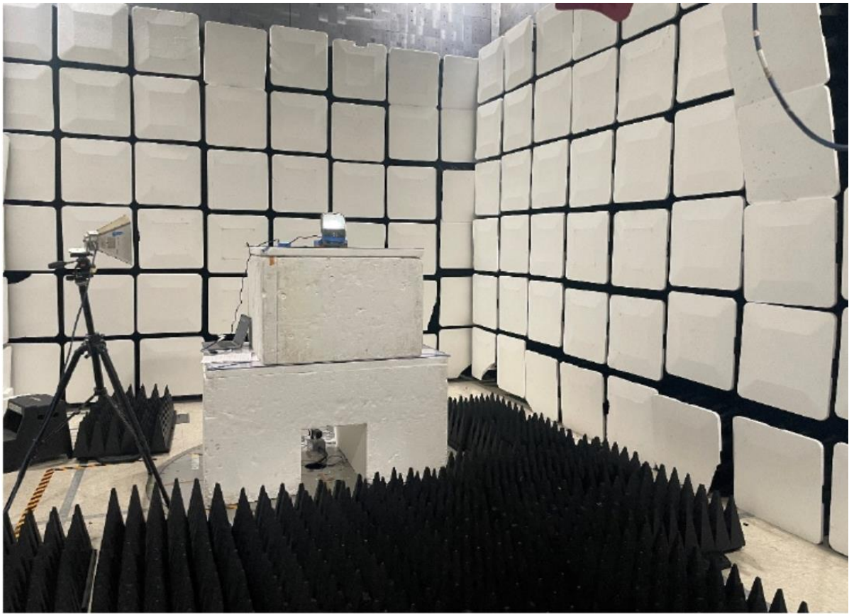
Figure 8.1.10 Radiated emissions 1-18 GHz (Front)
