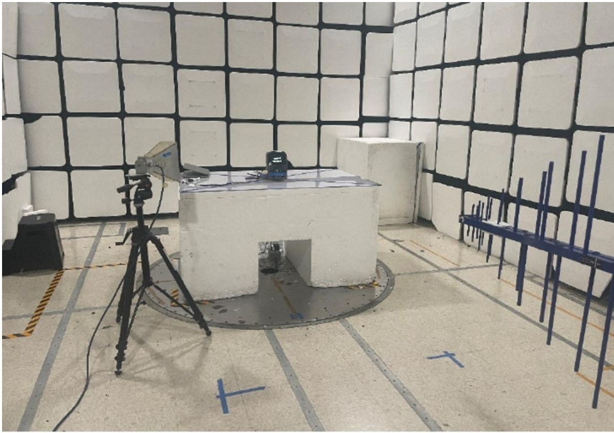
Figure 8.1.8 Radiated emissions 30-1000 MHz (Front)
