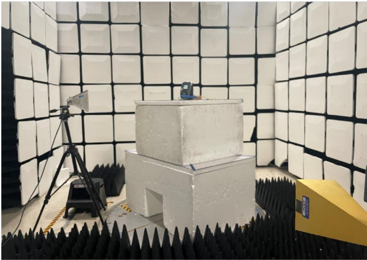
Figure 8.1.12 Radiated emissions 18-26.5 GHz (Front)
