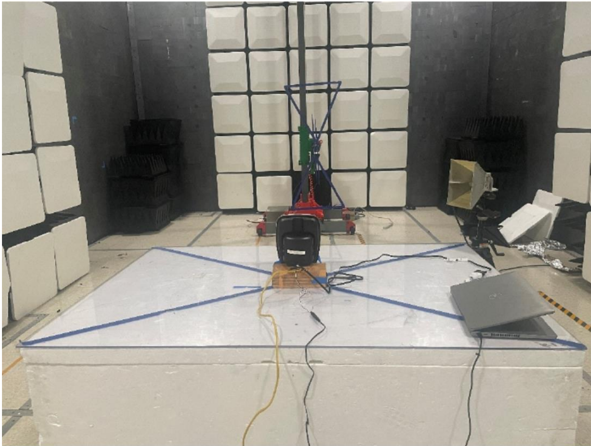
Figure 8.1.9 Radiated emissions 30-1000 MHz (Back)
