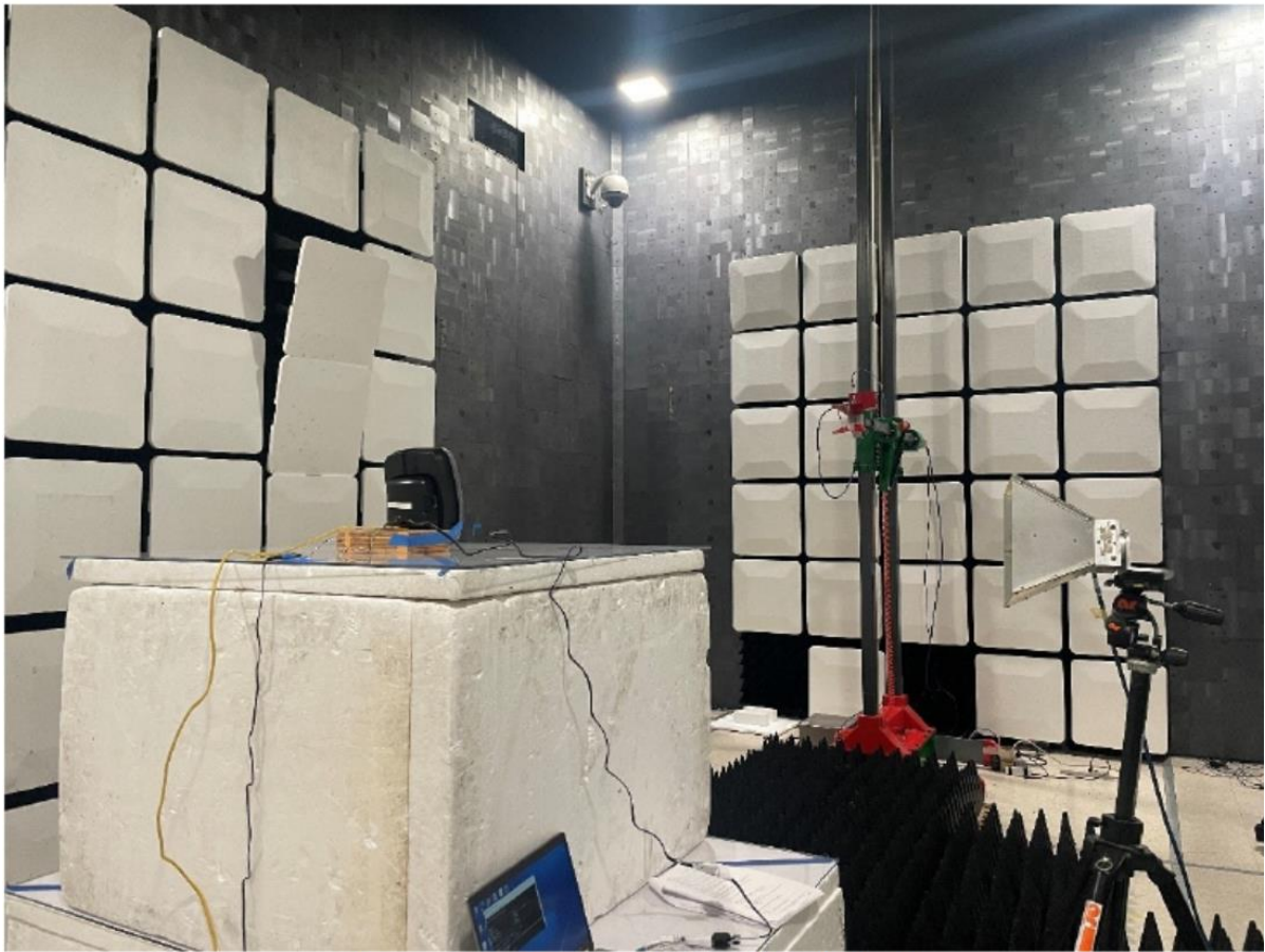
Figure 8.1.11 Radiated emissions 1-18 GHz (Back)
