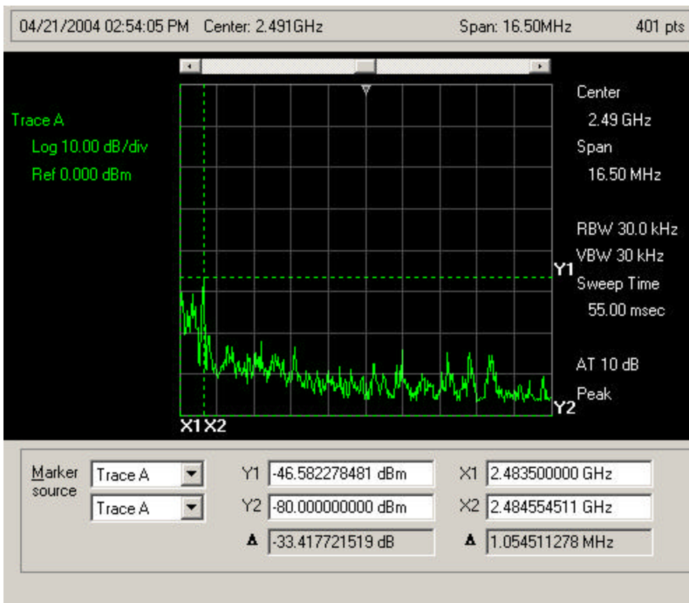
Plot 13: 2483.5 - 2500 MHz Restricted Band
