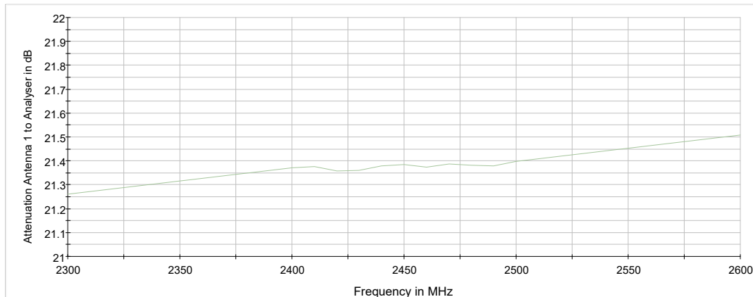
Attenuation Output power
