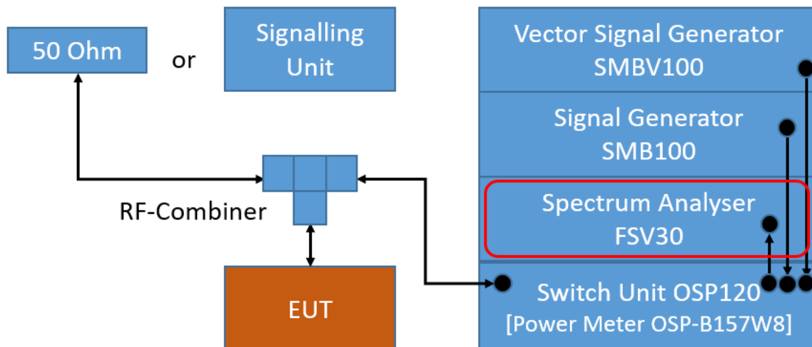
TS8997; Output Power
