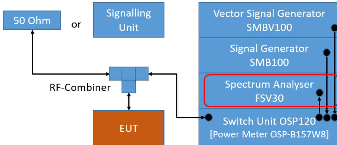
TS8997; Number of Hopping Frequencies
