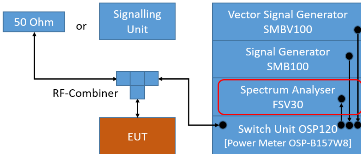
TS8997; Channel Separation
