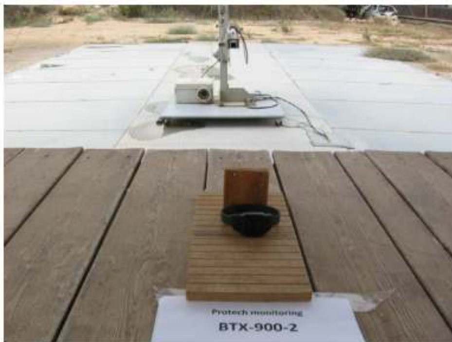
Figure 3. Radiated Emission Test 30-1000 MHz
