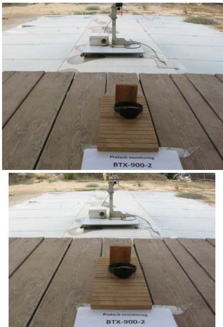
Figure 4. Radiated Emission Test Above 1 GHz
