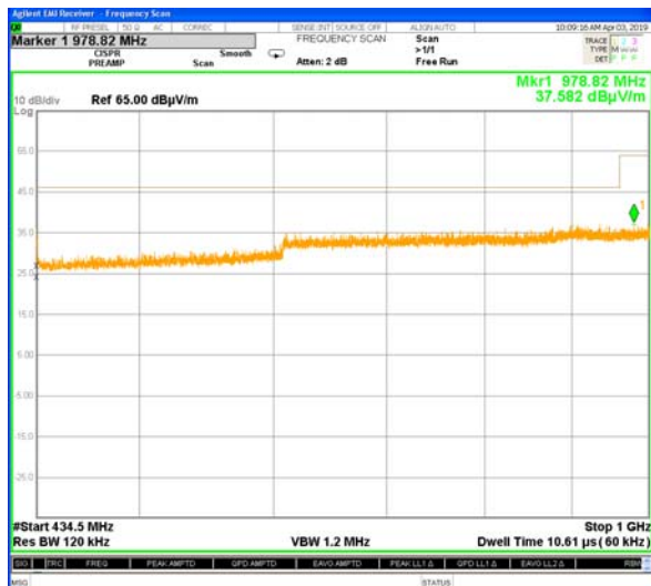
Plot # 4. Emissions scan 434.5 – 1000 MHz.
