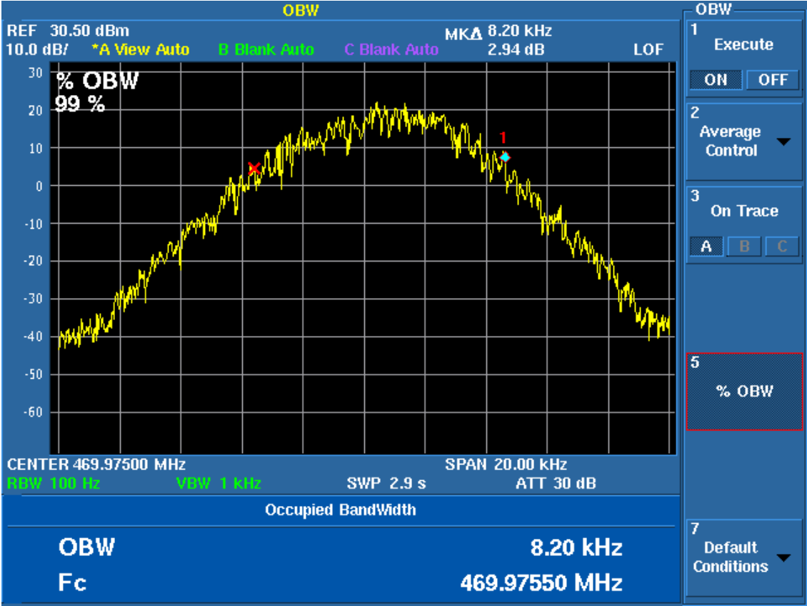
99% OBW 470 MHz
