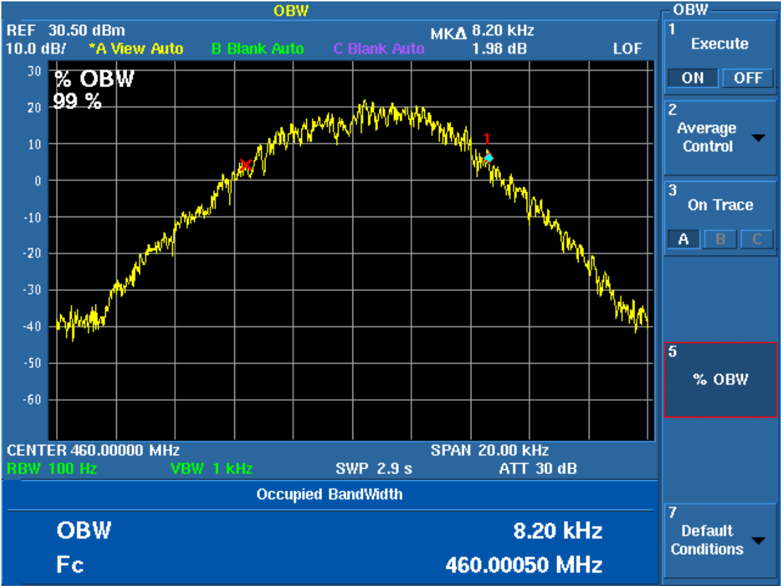
99% OBW 460 MHz
