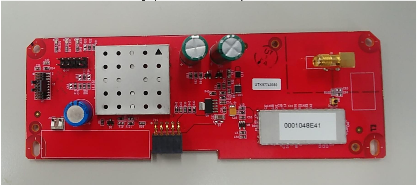
Photograph of RF Board: Shield removed
