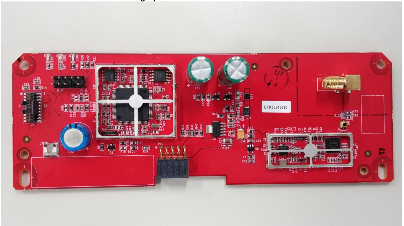
Photograph of RF Board: Shield removed
