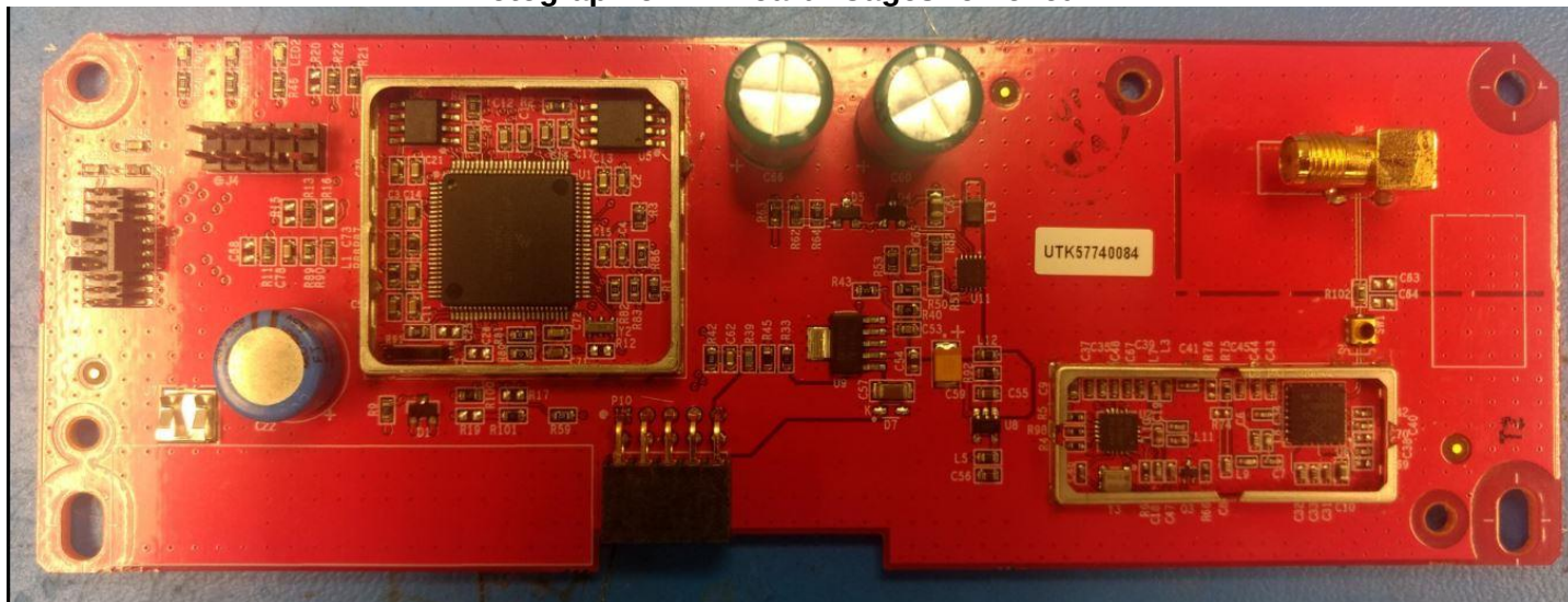
Photograph of RF Board: Foil Side
