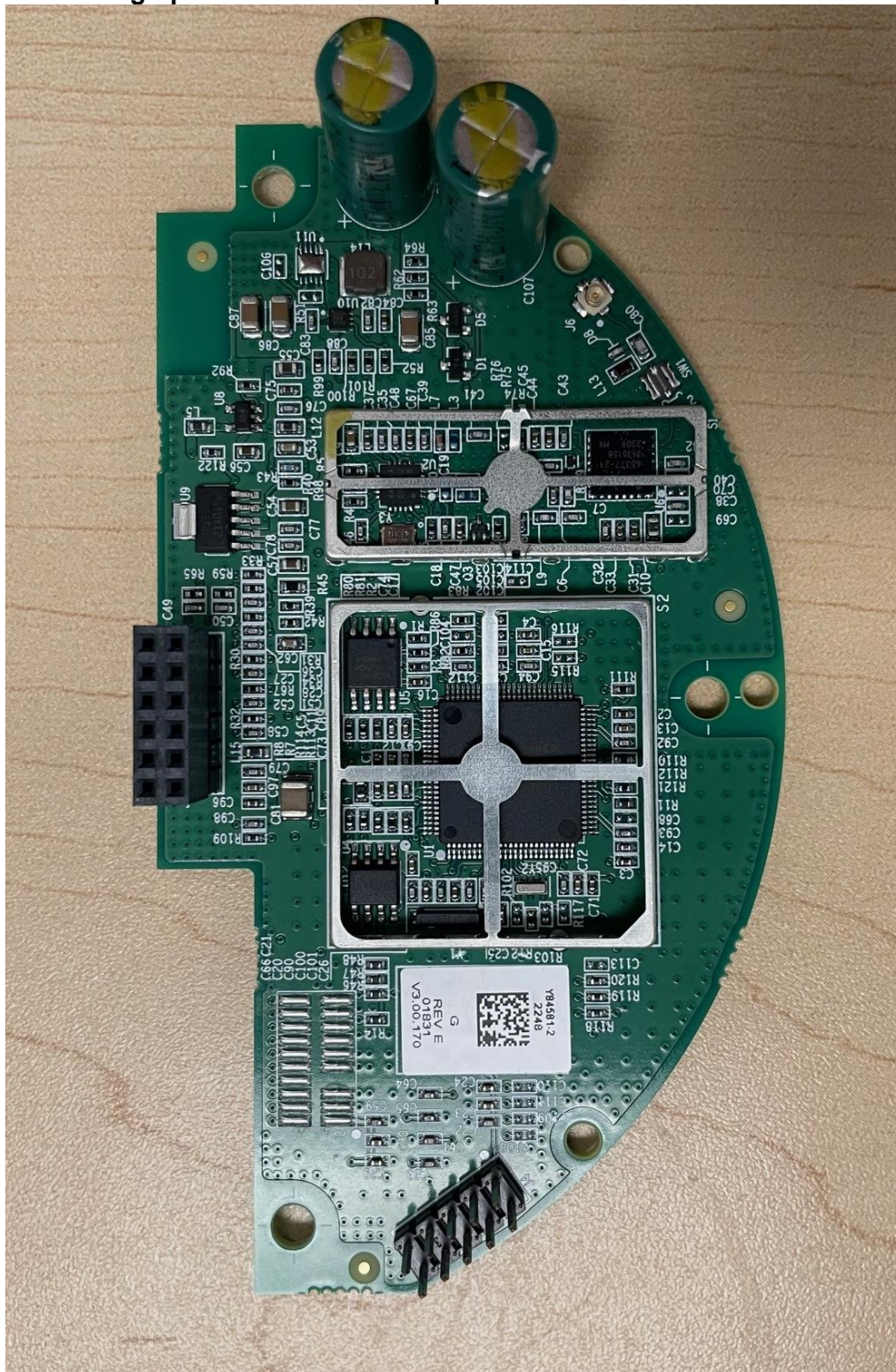
Photograph of PC Board: Component Side with shields removed
