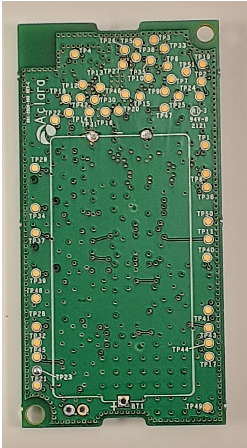
Photograph of PC Board foil side, battery removed
