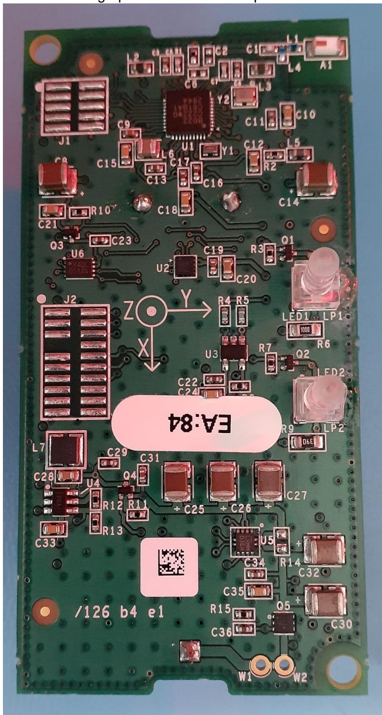
Photograph of PC Board: Component Side
