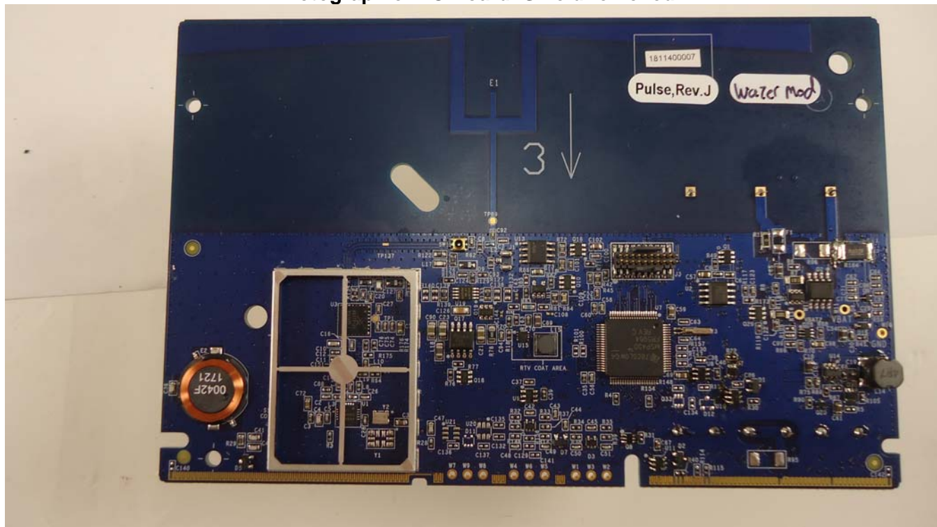
Photograph of PC Board: Shield removed
