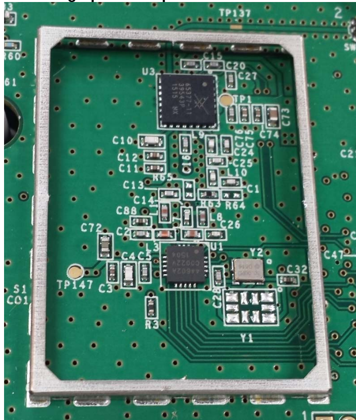
Photograph of components under the shield
