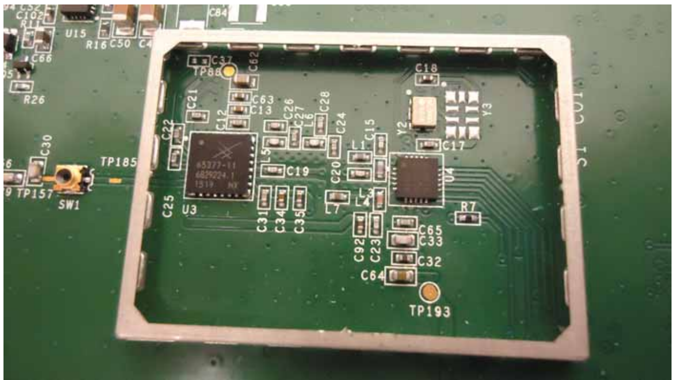
Photograph of PC Board: Component Side, Lower Shield removed
