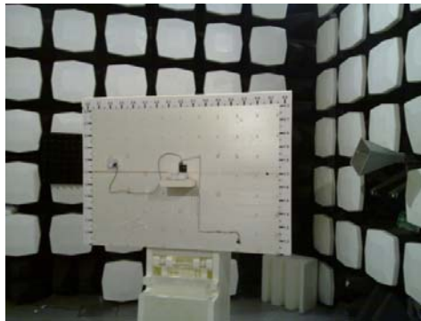
Above 30 MHz
