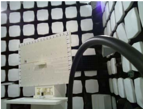
Below 30 MHz, Loop Antenna
