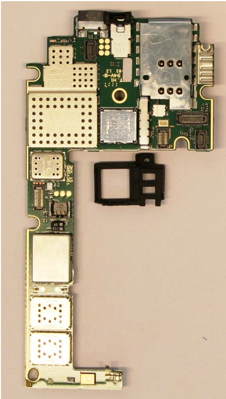
Internal Photos Exhibit 09 Applicant: Nokia Corporation
