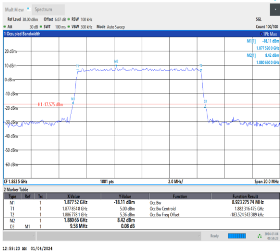
1-N25-15-10-M-5-DFT-256QAM-Outer_Full-50@0-A nt1-8.923-9.580-≤10-PASS
