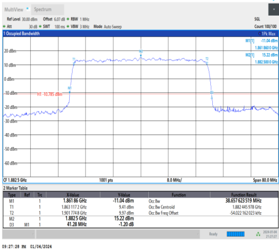
1-N25-15-40-M-7-CP-16QAM-Outer_Full-216@0-Ant 1-38.658-41.280-≤40-PASS
