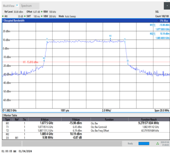
1-N25-15-10-M-7-CP-16QAM-Outer_Full-52@0-Ant1 -9.28-9.980-≤10-PASS
