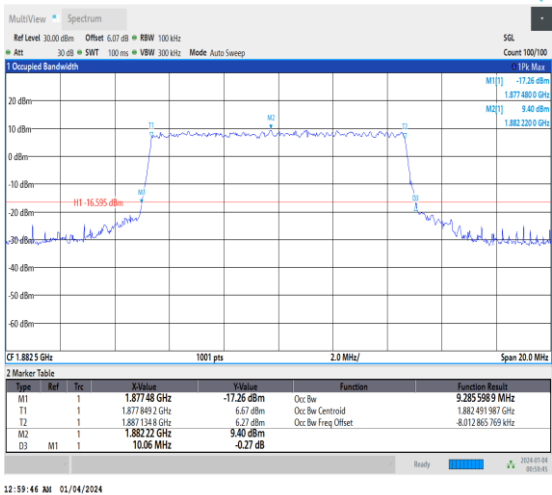
1-N25-15-10-M-6-CP-QPSK-Outer_Full-52@0-Ant1 9.286-10.060-≤10-PASS
