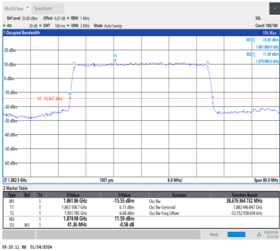
1-N25-15-40-M-9-CP-256QAM-Outer_Full-216@0-A nt1-38.676-41.360-≤40-PASS
