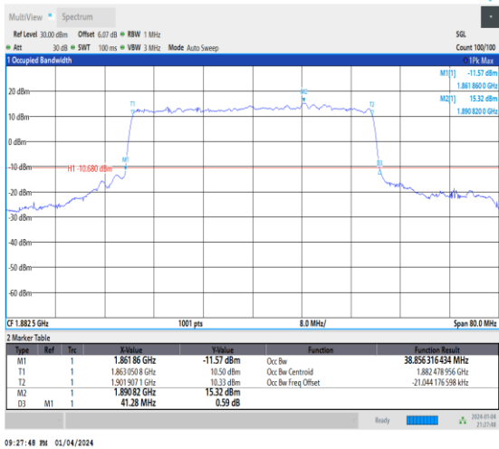
1-N25-15-40-M-8-CP-64QAM-Outer_Full-216@0-Ant 1-38.856-41.280-≤40-PASS
