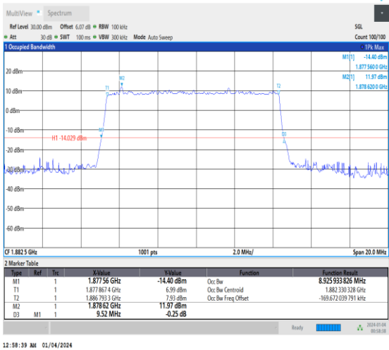
1-N25-15-10-M-4-DFT-64QAM-Outer_Full-50@0-Ant 1-8.926-9.520-≤10-PASS
