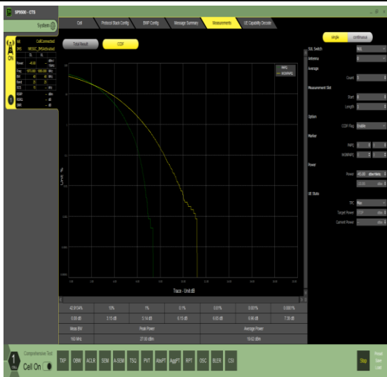
1-N25-PC3-15-40-H-15-NS_01-CP-256QAM-Outer_ Full-216@0-6.15
