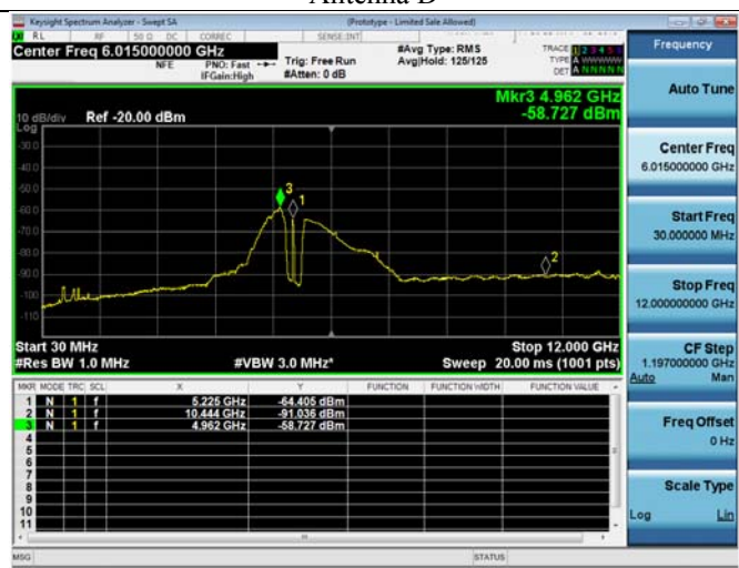
Antenna D
