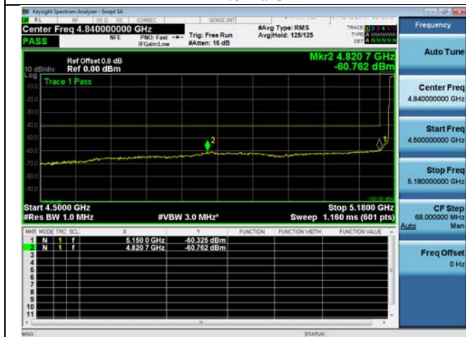
Antenna C
