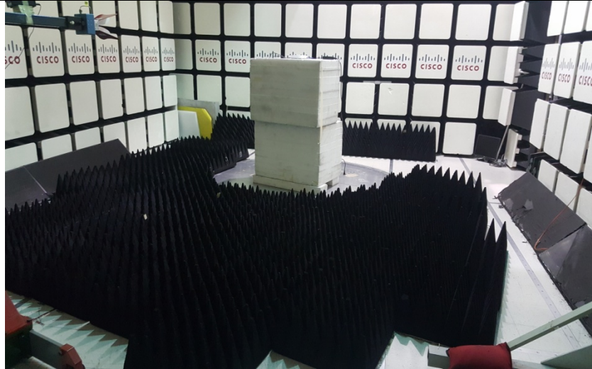
Radiated Setup 1GHz – 18GHz
