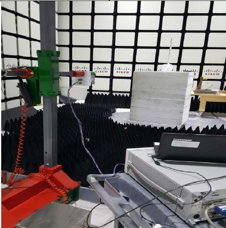
Radiated Setup 18GHz – 26GHz
