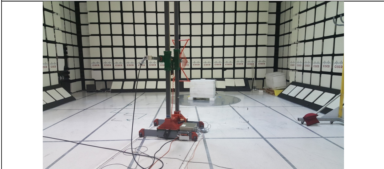
Radiated Setup 30MHz – 1GHz
