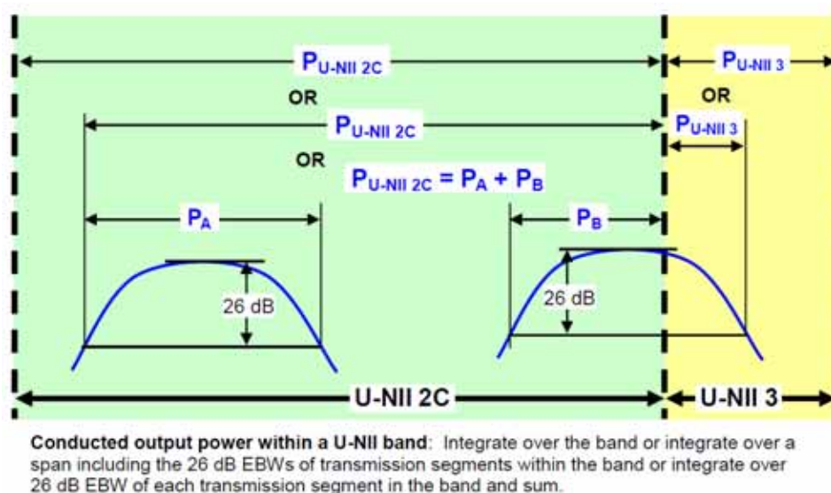
Figure 4. Conducted Output Power Measurement Examples
