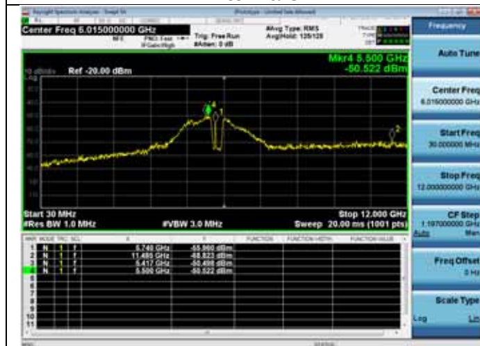
Antenna C
