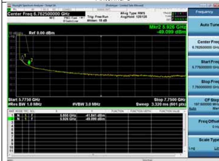
Antenna C
