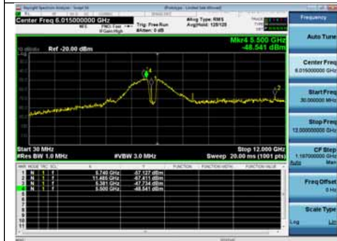
Antenna C
