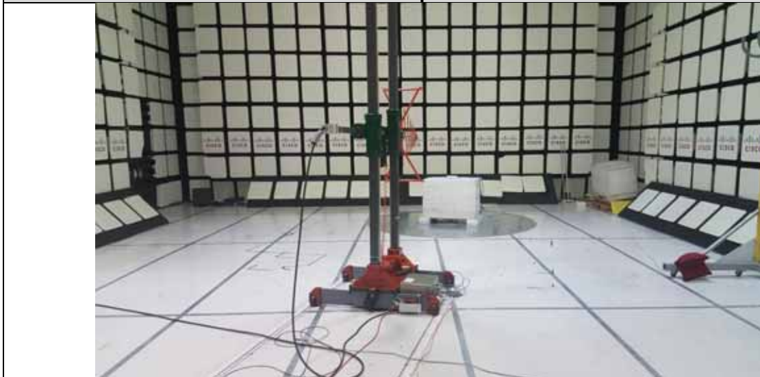
Radiated Setup 30MHz – 1GHz
