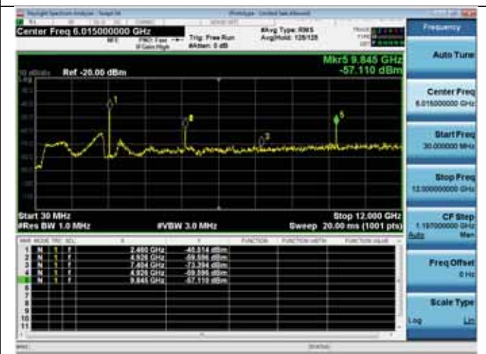
Antenna D
