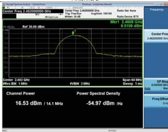
Antenna D
