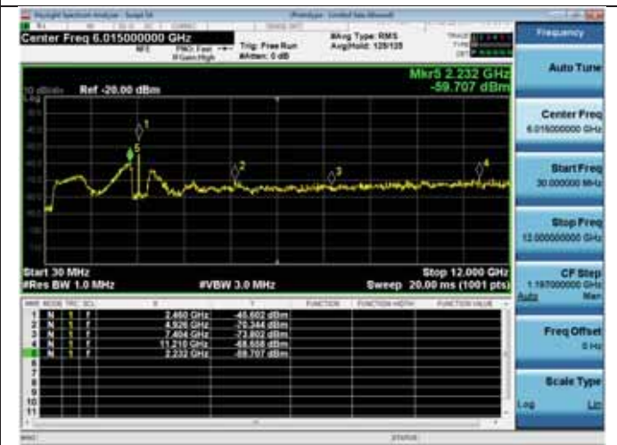
Antenna D
