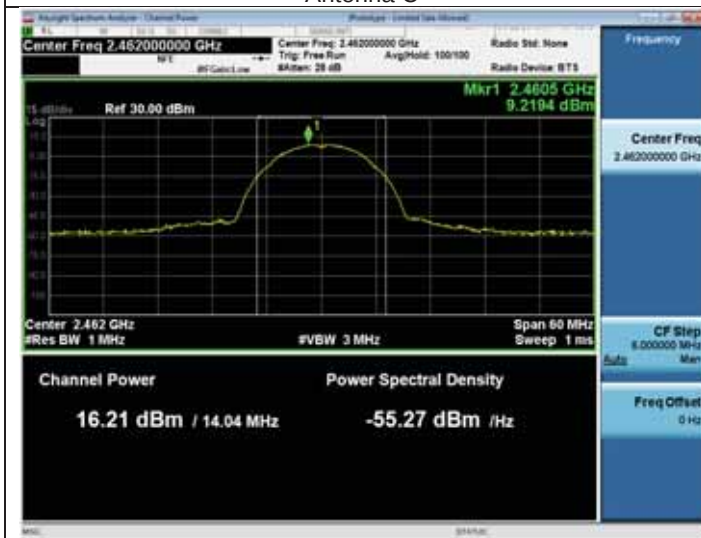
Antenna C
