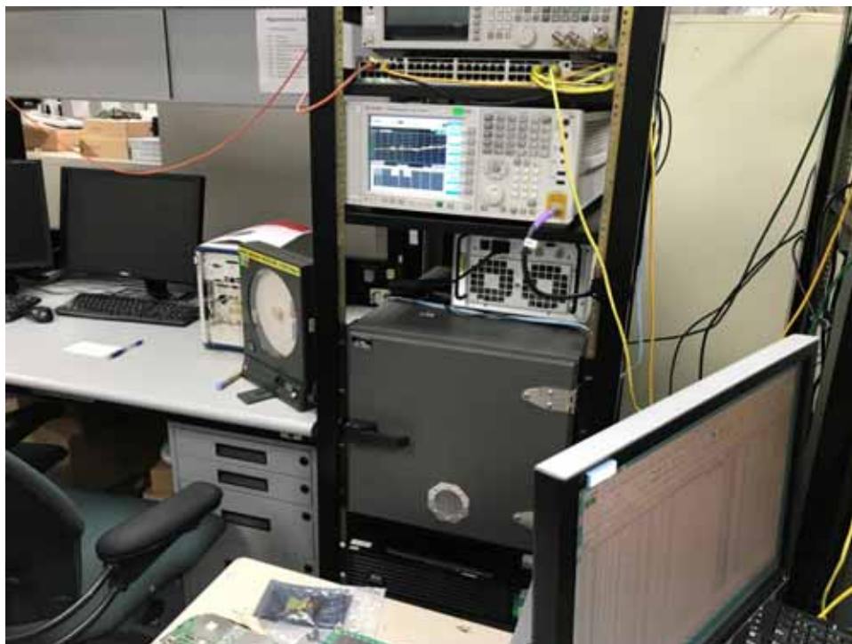
Title: Radio Conducted Test Setup
