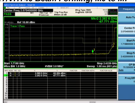
Antenna B
