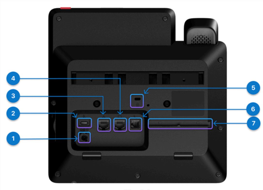
Figure 8. Cisco Desk Phone 9861 back view
