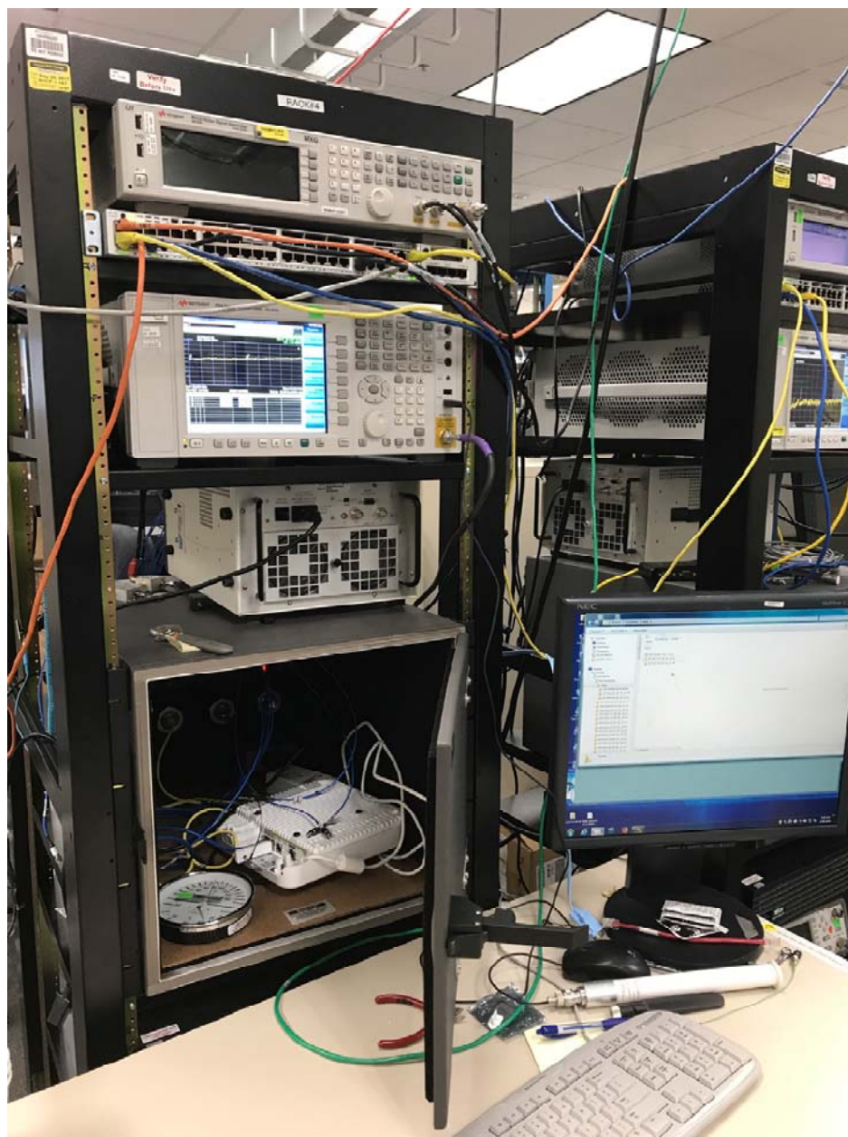
Title: Radio Conducted Test Setup.
