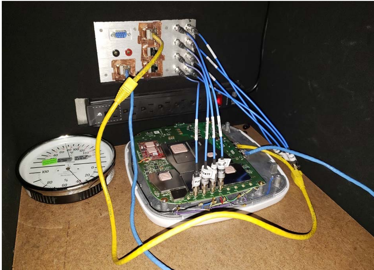
Title: Radio Conducted Test Setup
