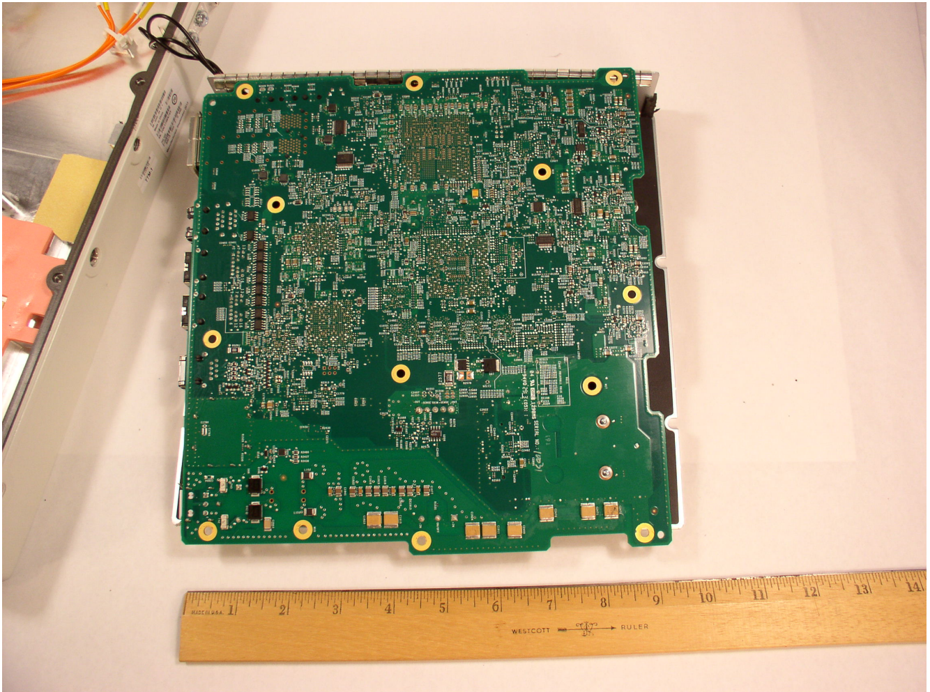
Internal- PCB mains board of ASR901 router (Bottom)
