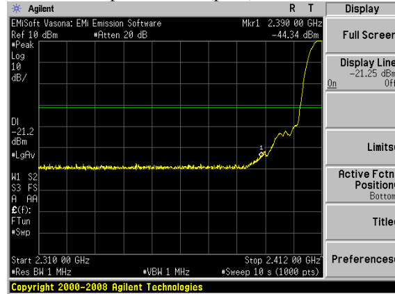
802.11B 1Mbps channel 1 (peak)
