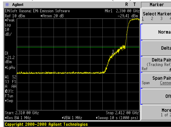
802.11N, Mcs M0 rate channel 1 (Peak)
