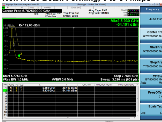
Antenna B
