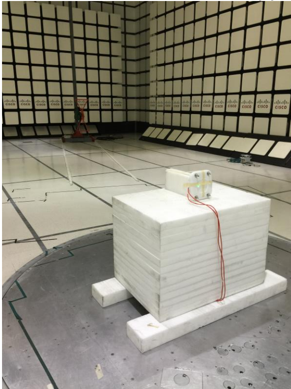
AIR-CAP2702E-B-K9 Radiated Test setup photo above 1GHz
