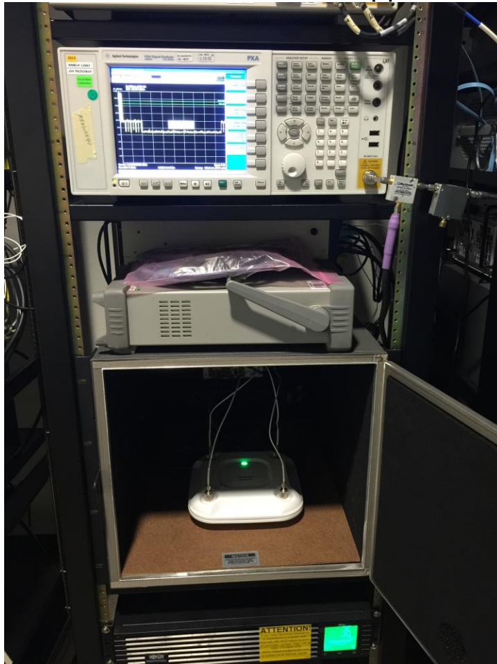
AIR-CAP2702E-B-K9 Conducted Test setup photo
