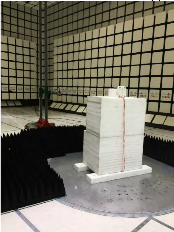
AIR-CAP2702E-B-K9 Radiated Test setup photo above 1GHz
