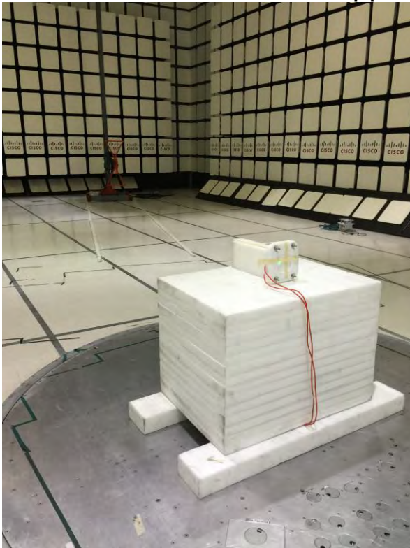
AIR-CAP2702E-B-K9 Radiated Test setup photo 30MHz to 1GHz
