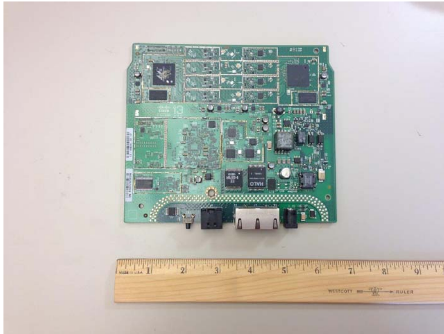
Unshielded Board Top
