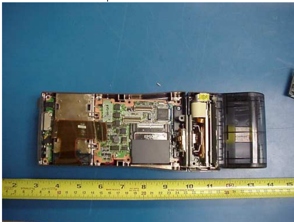
Top View Of The Bottom Part
