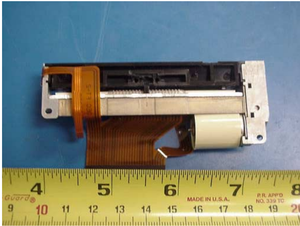
Bottom View Of Printer
