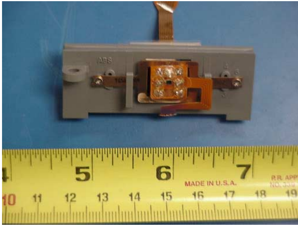
Bottom View Of Flex
