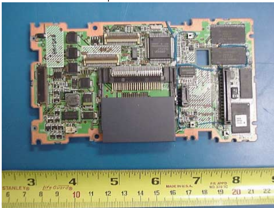
Top View Of The Board
