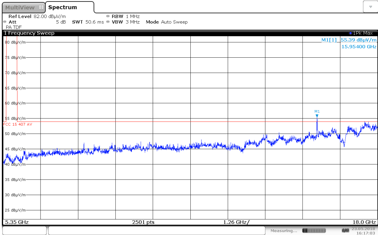
Radiated Emissions, 5350 – 18000 MHz, 5320 MHz, 802.11n HT20, MIMO, HP
