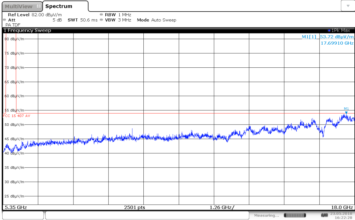
Radiated Emissions, 5350 – 18000 MHz, 5240 MHz, 802.11n HT20, MIMO, HP
