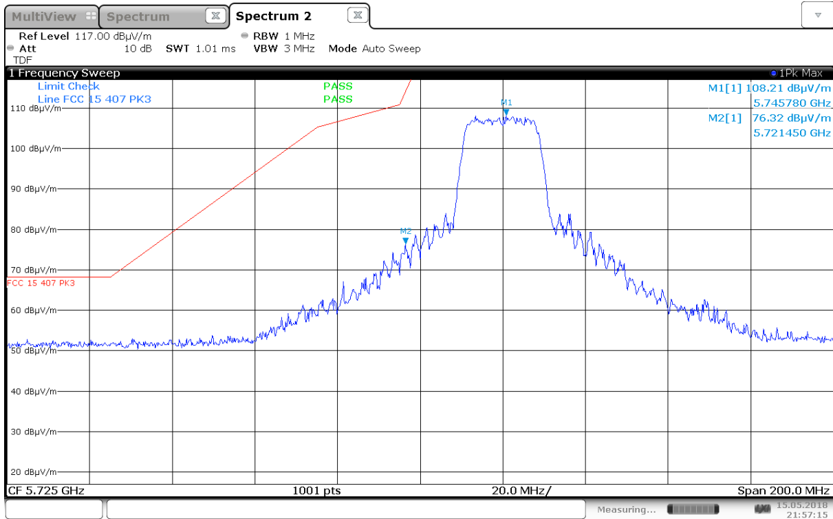
Unwanted Emissions, Band Edge, 5725MHz, ch149, 802.11n MCS0 HT20, MIMO
