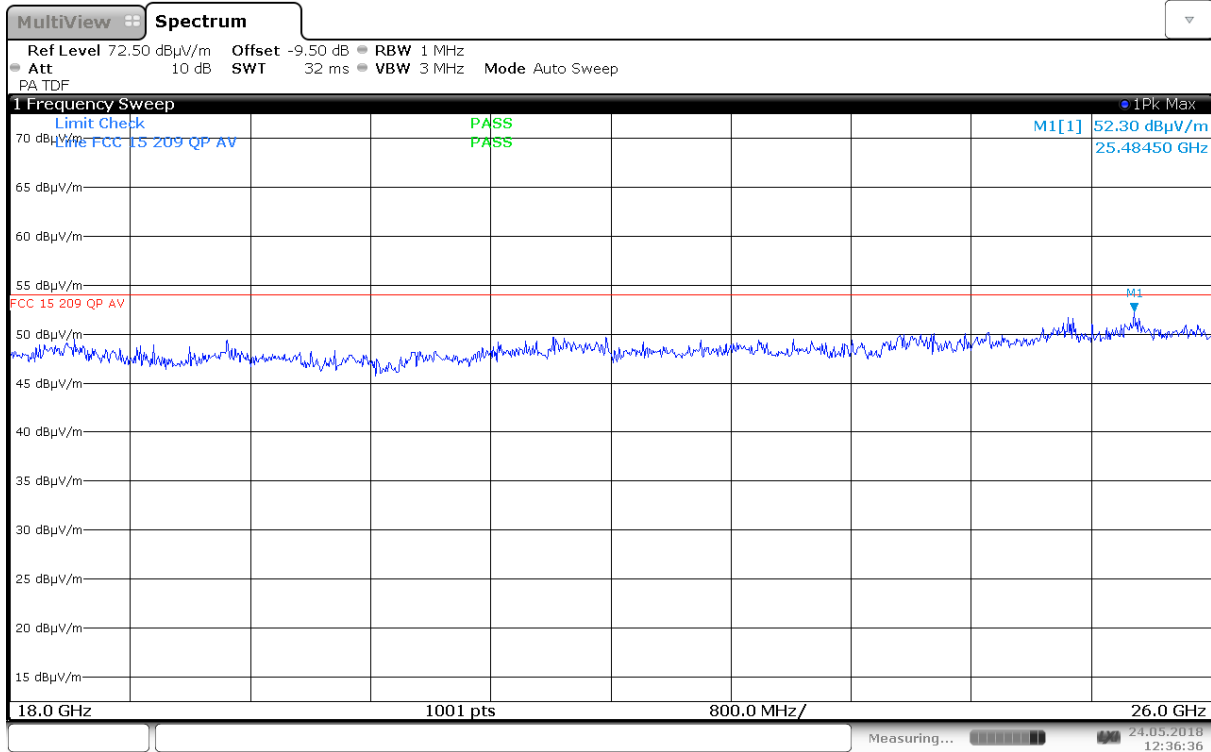
Radiated Emissions, 18.0 – 26.0GHz, 5580 MHz, 802.11a 6M, Ant 0, HP, @1m
