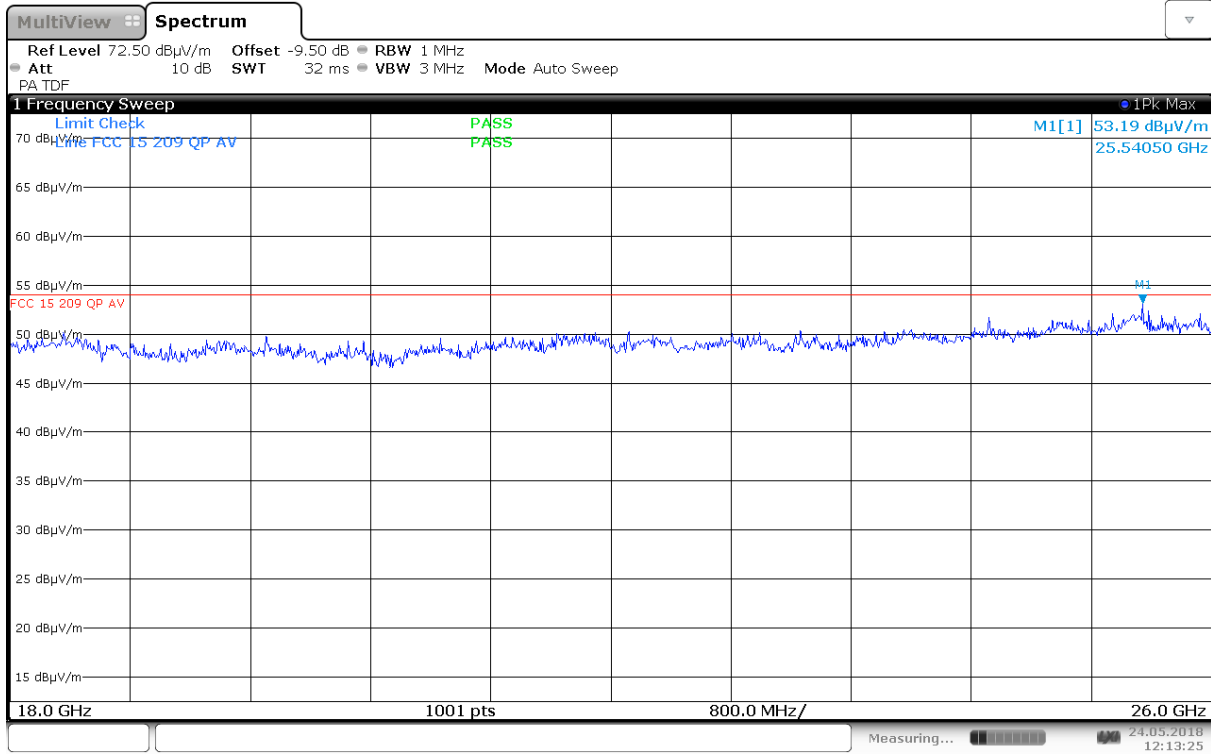
Radiated Emissions, 18.0 – 26.0GHz, 5300 MHz, 802.11a 6M, Ant 0, HP, @1m
