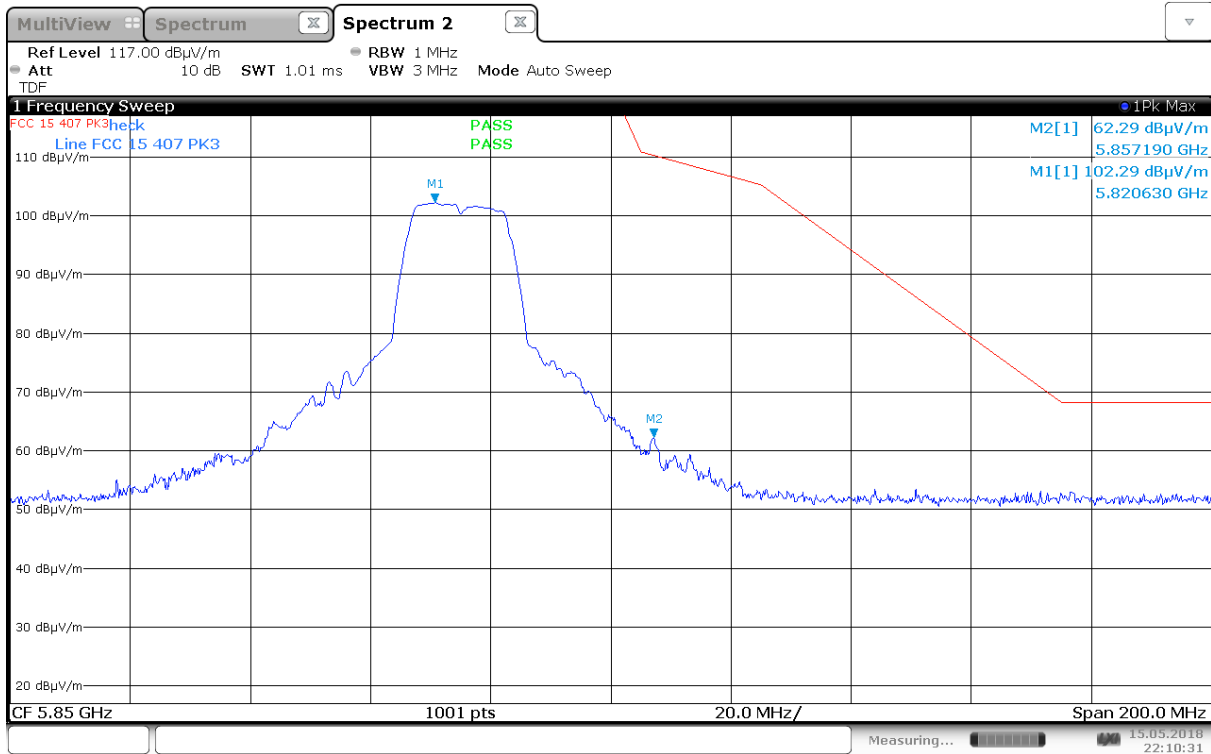
Unwanted Emissions, Band Edge, 5850MHz, ch165, 802.11a 6M, ant 0
