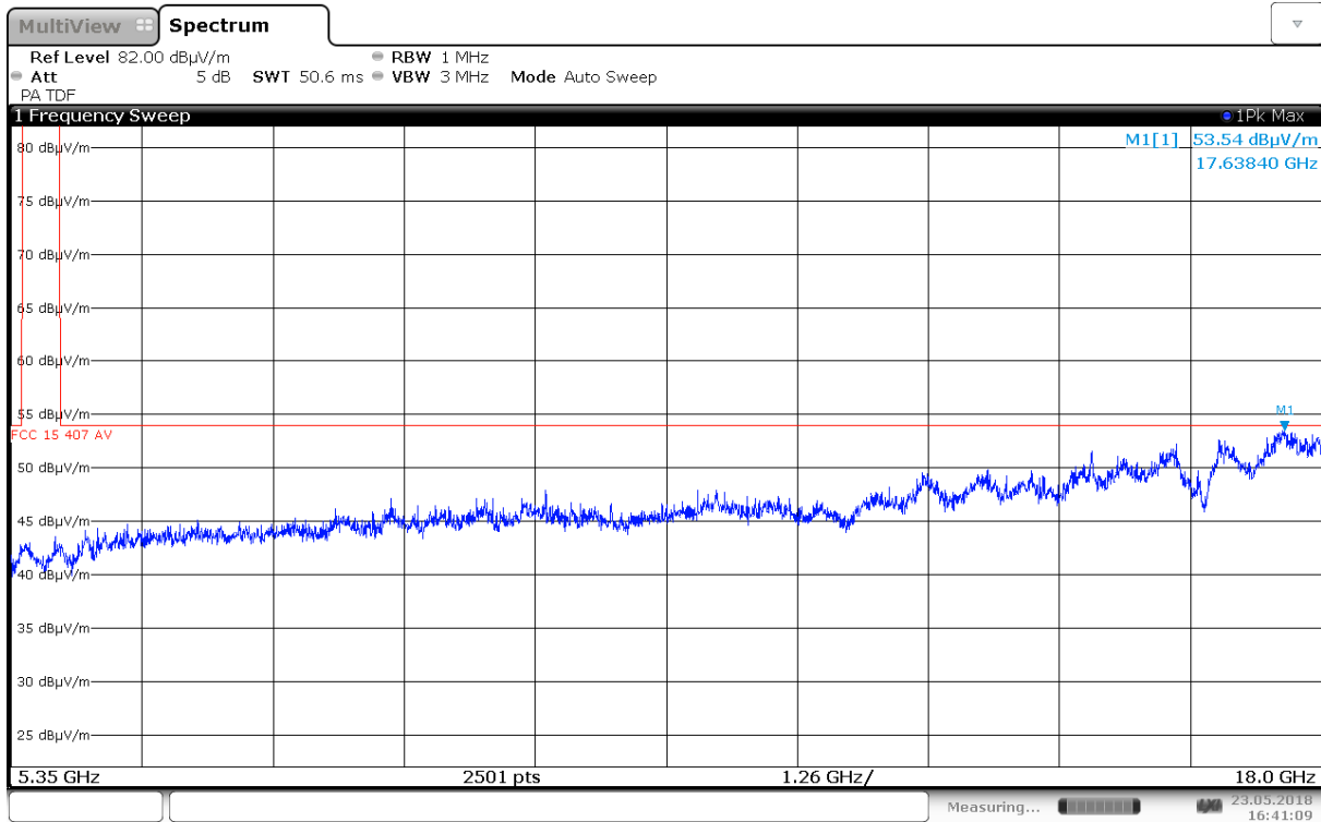
Radiated Emissions, 5350 – 18000 MHz, 5260 MHz, 802.11a 6M, Ant0, HP
