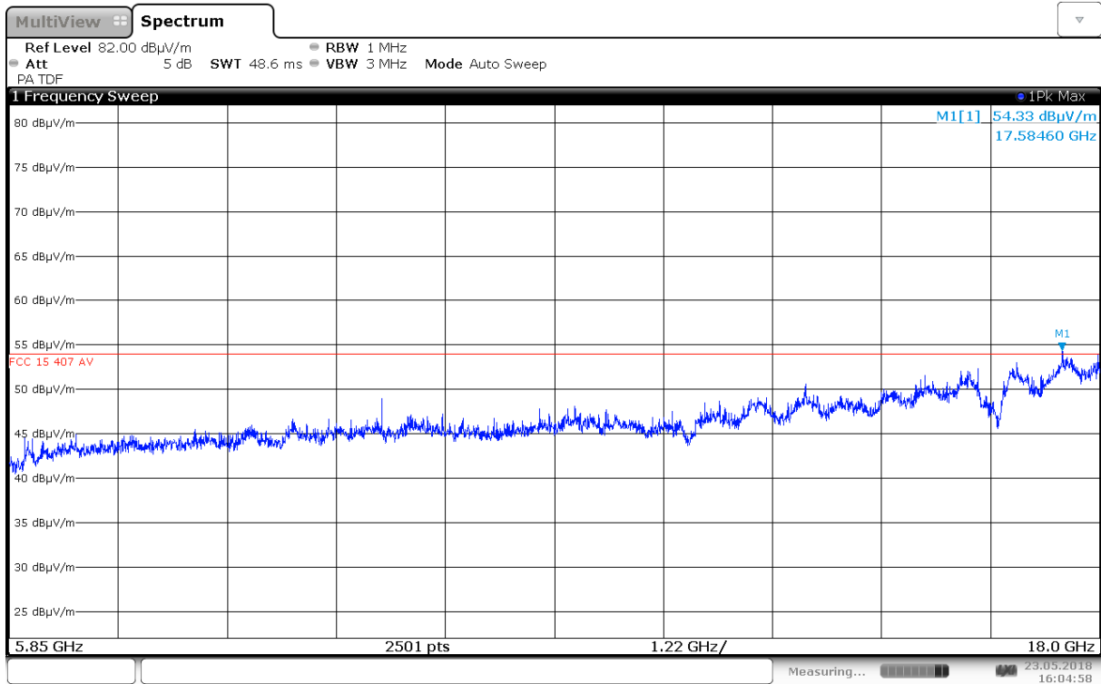
Radiated Emissions, 5850 – 18000 MHz, 5700 MHz, 802.11n HT20, MIMO, HP
