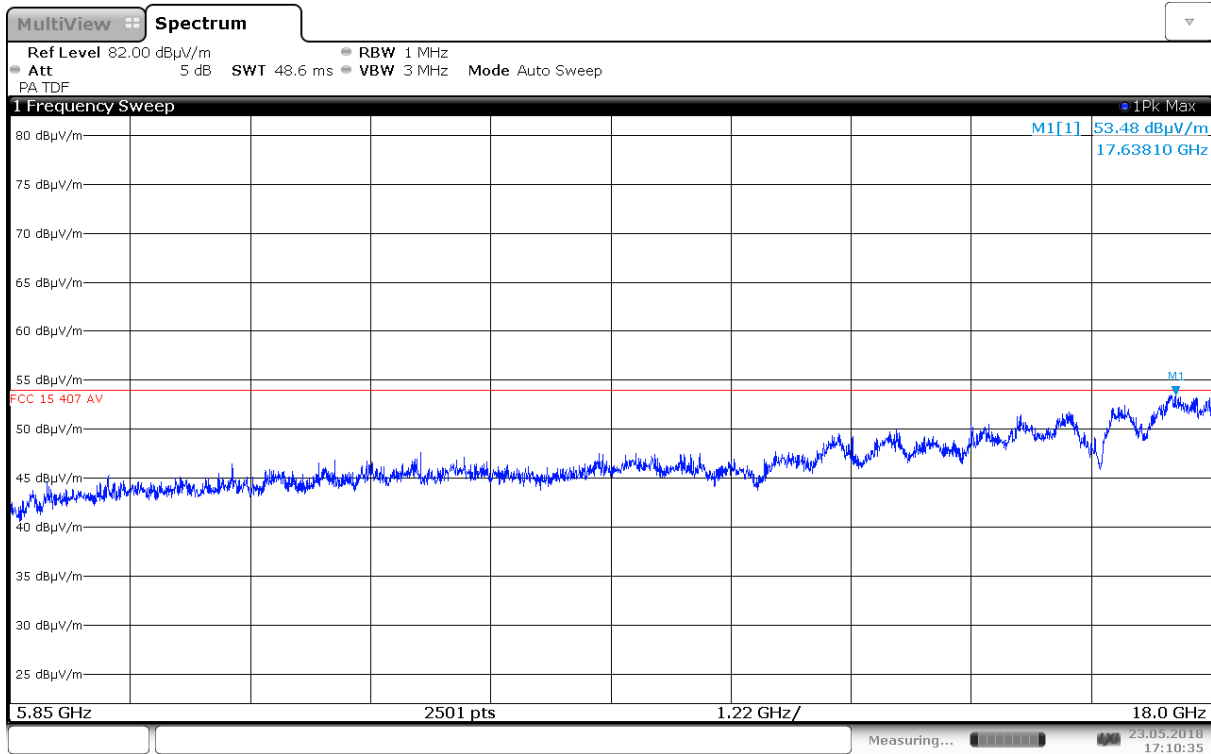
Radiated Emissions, 5850 – 18000 MHz, 5785 MHz, 802.11a 6M, Ant1, HP
