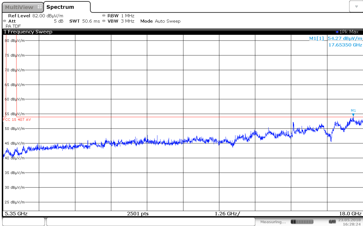
Radiated Emissions, 5350 – 18000 MHz, 5180 MHz, 802.11a 6M, Ant0, HP
