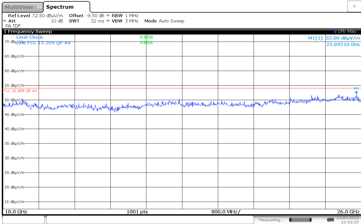
Radiated Emissions, 18.0 – 26.0GHz, 5580 MHz, 802.11a 6M, Ant 1, HP, @1m
