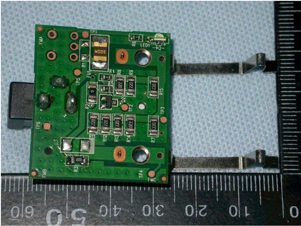
12. Rear view of PCB
