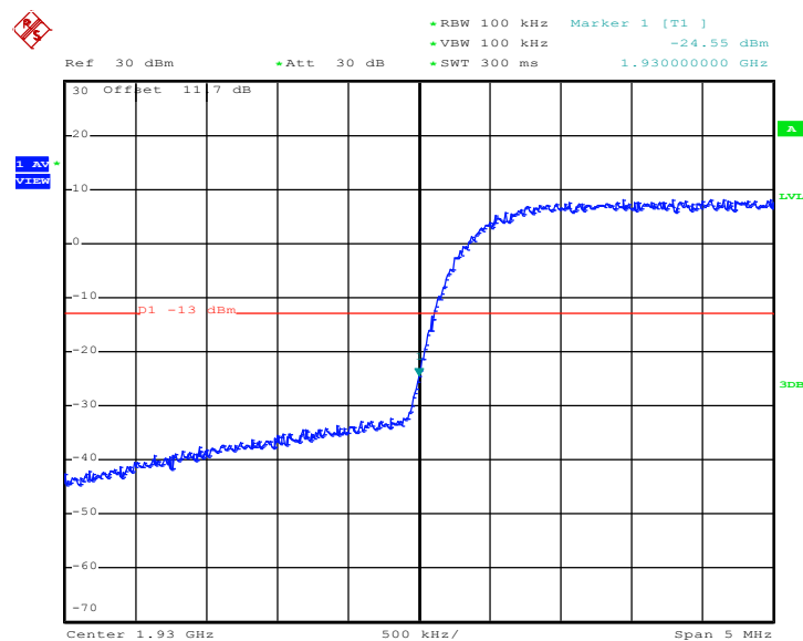
Lower Band Edge Plot on Channel 9662 (1932.4 MHz)
