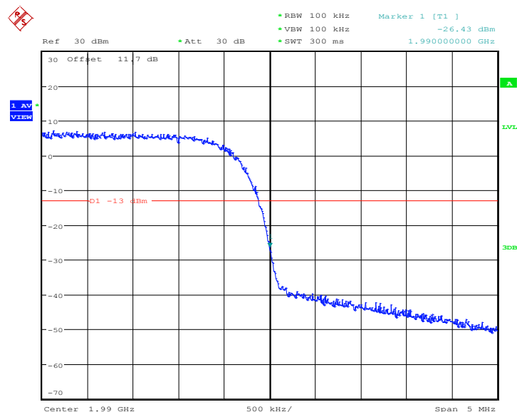
Higher Band Edge Plot on Channel 9938 (1987.6 MHz)
