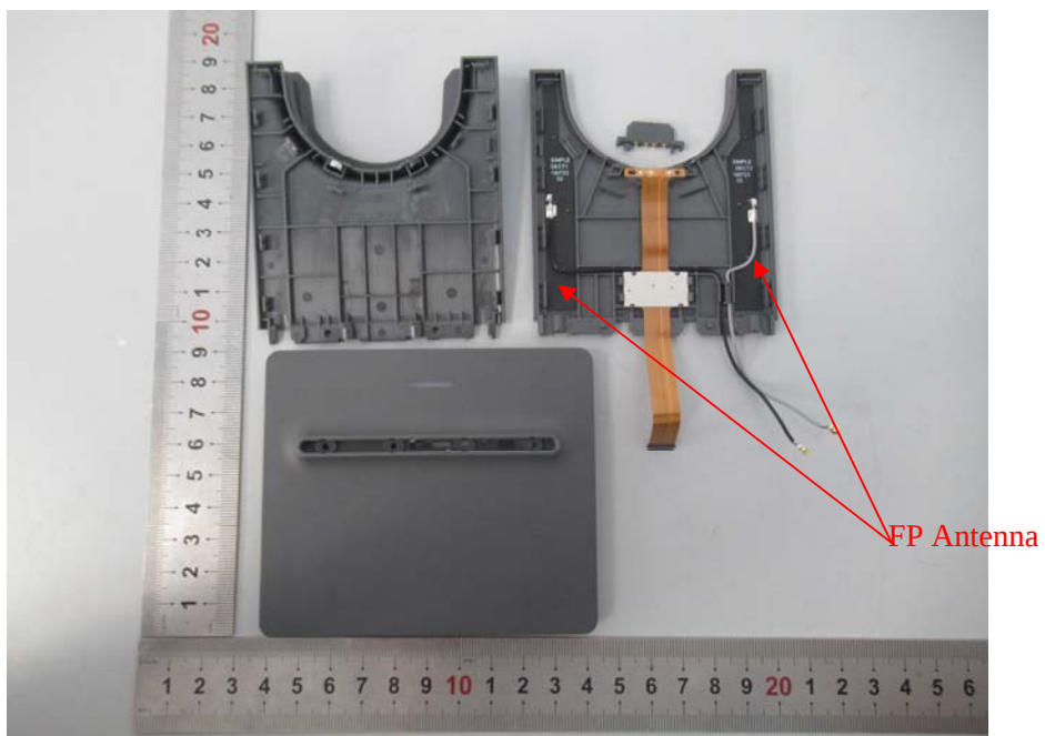
EUT – Antenna View
