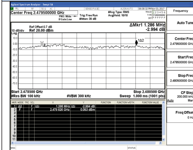
Channel 78 / 2480 MHz
