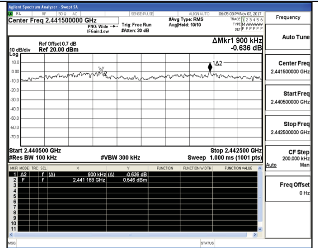
Channel 39 / 2441 MHz
