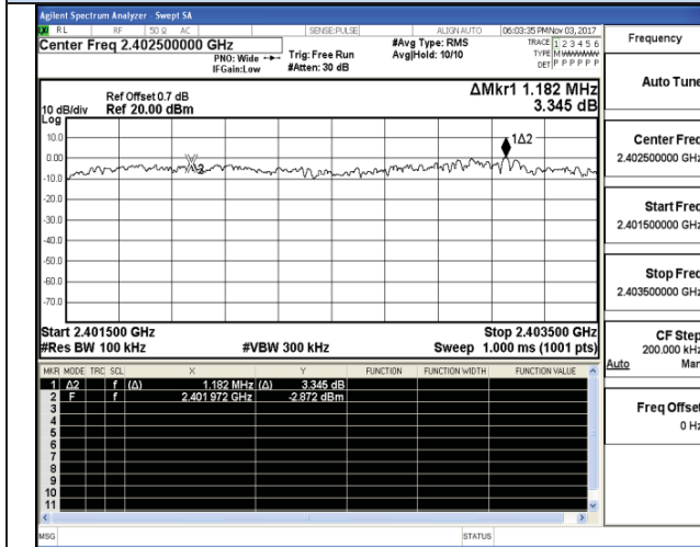
Channel 0 / 2402 MHz
