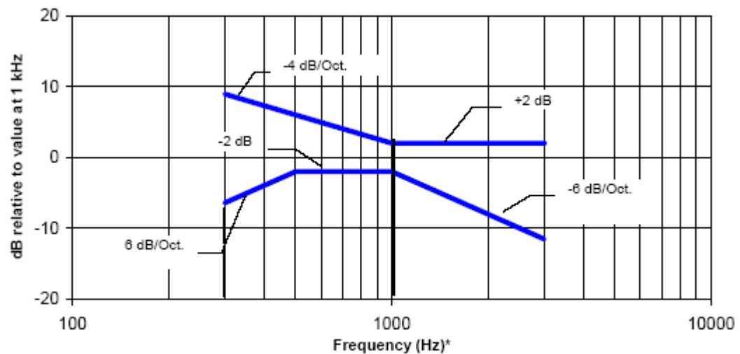
Figure 6.5-3 Magnetic field frequency response for WDs with a field between 10 dB and -13 dB (A/m) at 1 kHz
