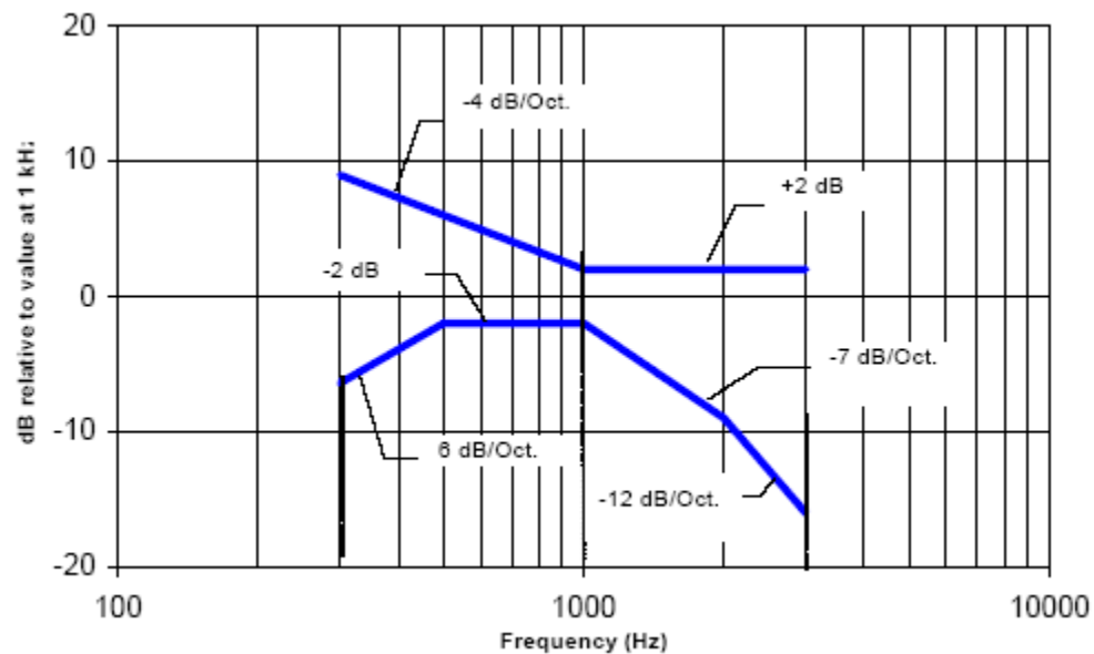
Figure 6.5-4 Magnetic field frequency response for WDs with a field that exceeds -10 dB(A/m) at 1 kHz
