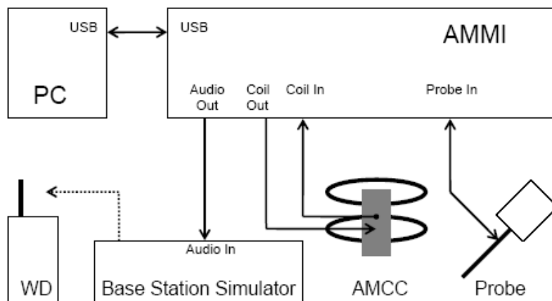
Figure 5.0-3. T-Coil set up cabling
