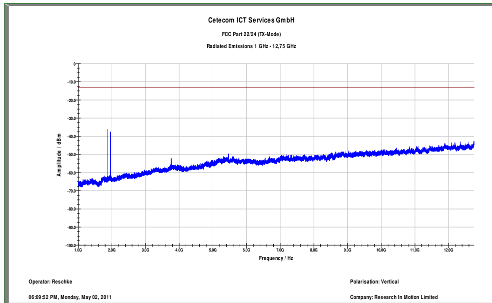
Plot 10: Channel 9400 (1 GHz – 12.75 GHz) – vertical
