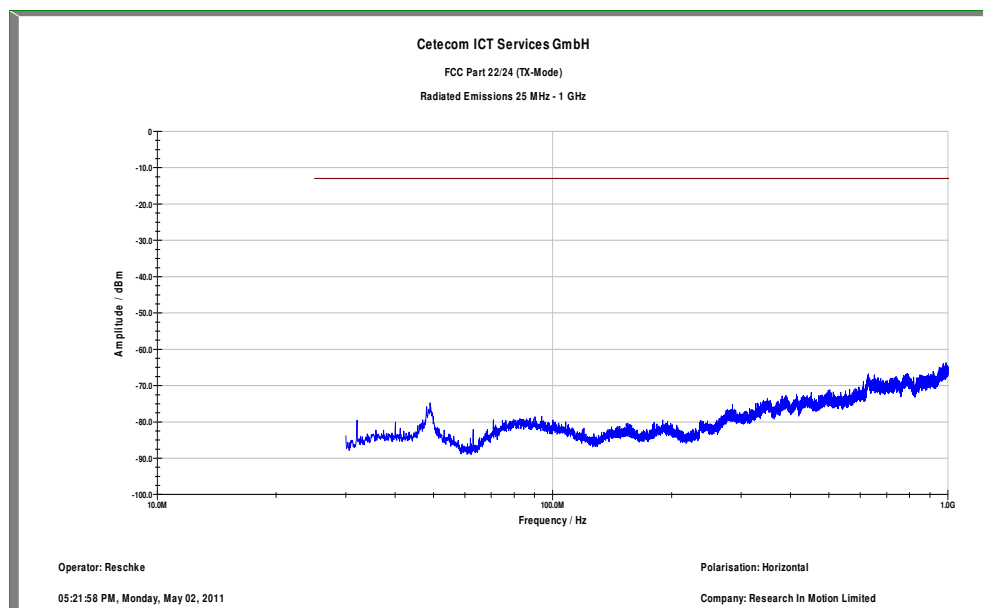
Plot 6: Channel 9262 (30 MHz - 1 GHz) – horizontal
