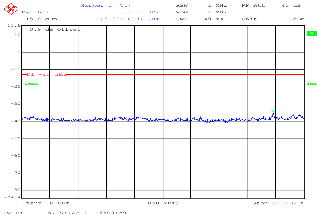
Plot 19: Channel 9538 (18 GHz - 26.5 GHz) – vertical/horizontal (max hold)
