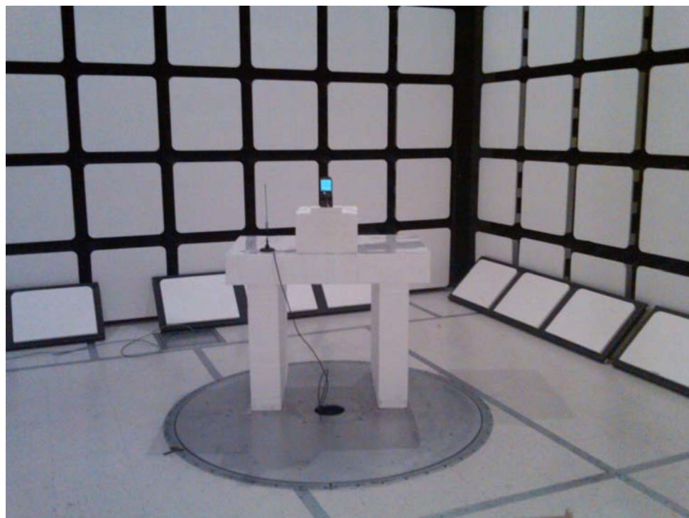
Radiated Unintentional Emissions Test-Setup Photos cont'd
