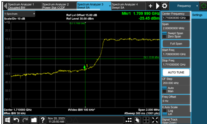
FULL CH 131997 (1712.5 MHz)
