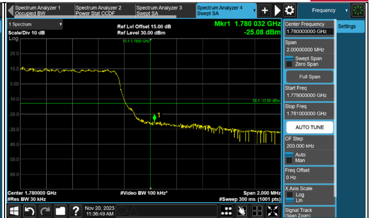
FULL CH 132647 (1777.5 MHz)
