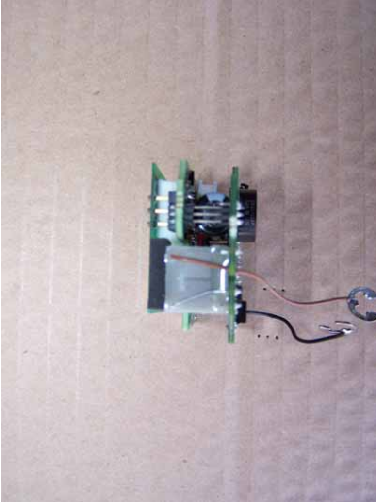
Assembled Collar Unit PCB's
