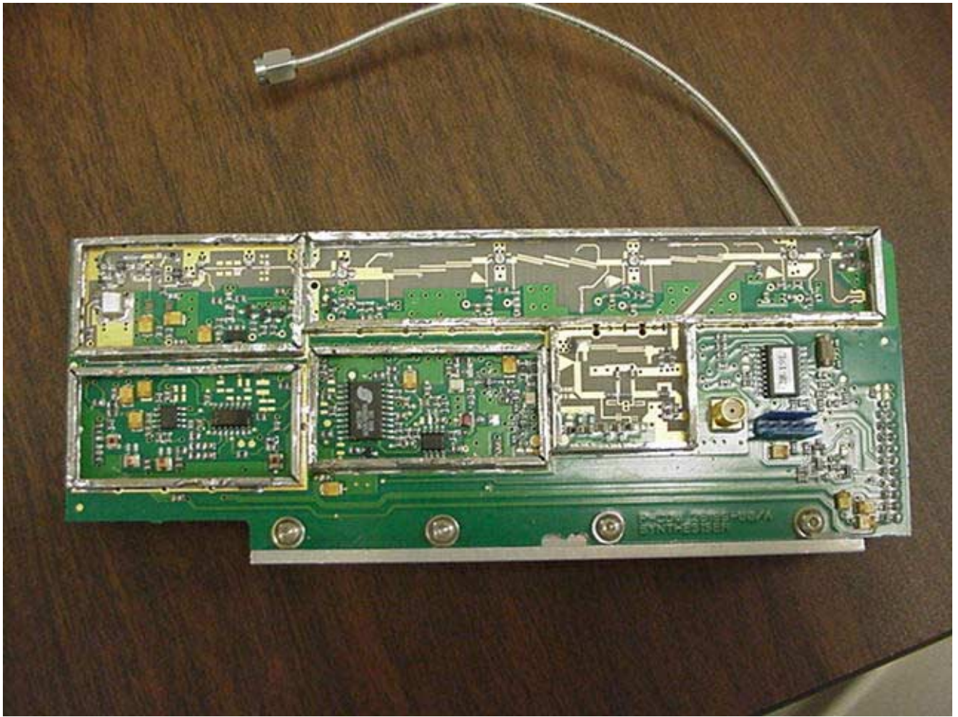
Synthesizer Board Top Side
