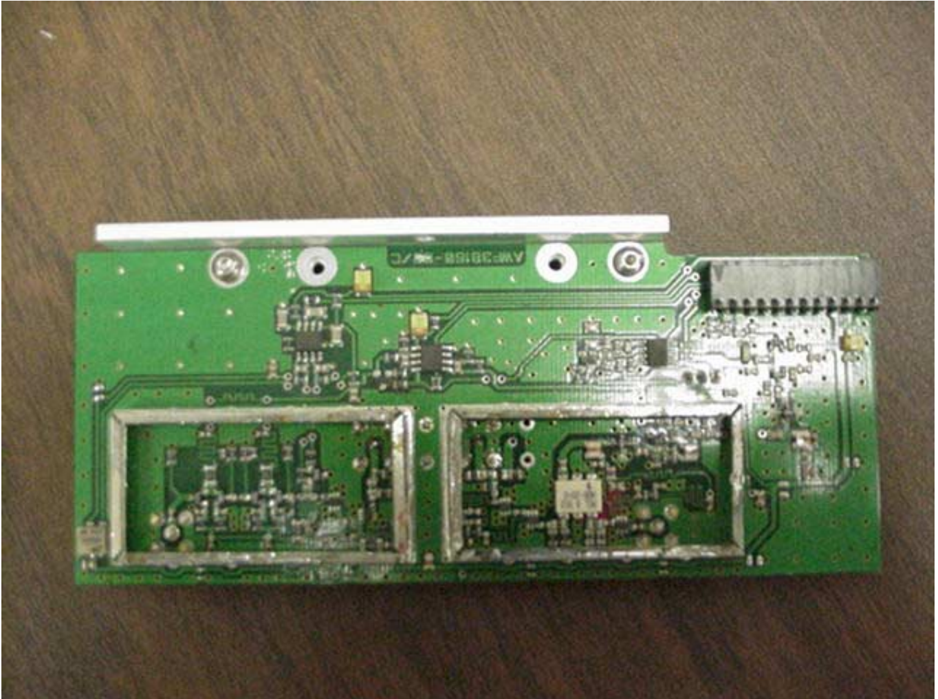
TX IF Board, Top Side
